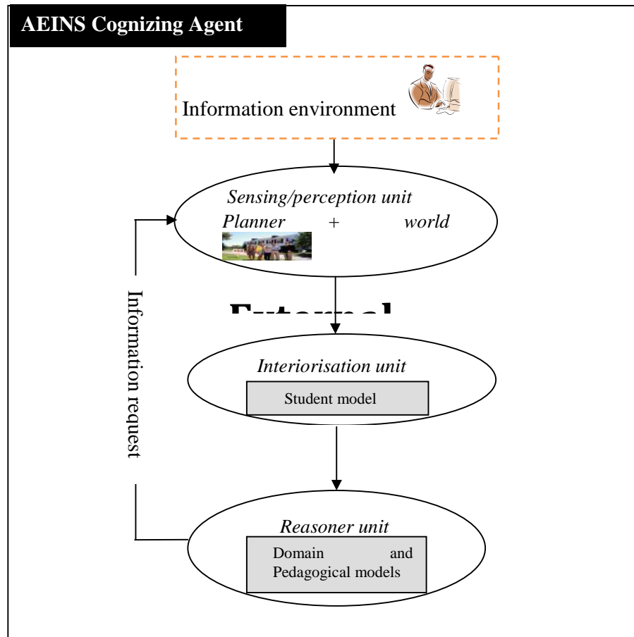
Fig.2: AEINS-CA architecture
