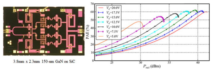
Fig. 10. 10-GHz class-E MMIC PA for supply modulation [9].
