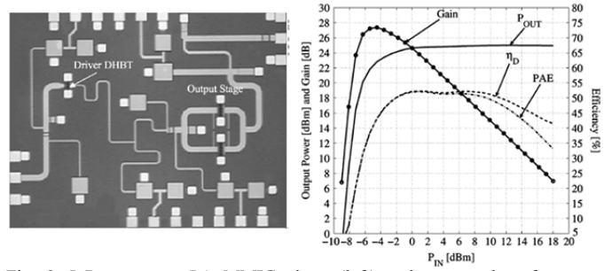
Fig. 8. InP two-stage PA MMIC photo (left) and measured performance (right) [6]. The MMIC is 2.65mm x 2.1mm in size.
