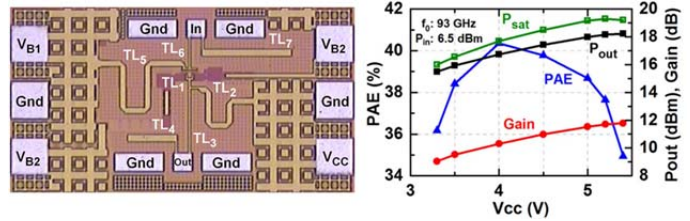
Fig. 9. Bi-CMOS W-band class-E MMIC photo and performance [11].
