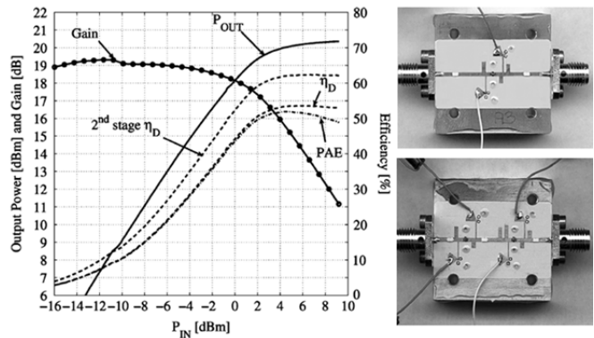
Fig. 5. Photographs of the output stage only (top right) of a hybrid class-E 10-GHz GaAs PA with PAE=62%, and a two-stage class-E PA with both stages operating close to class-E (bottom). The plots show measured data for the two-stage PA calibrated at the SMA connectors [6].
