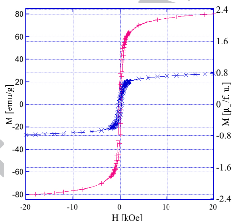
Figure 5. (Color online) Isothermal magnetization hysteresis loops at 5 K for the core-only sample (+) and for the multi-core-shell sample (x).
