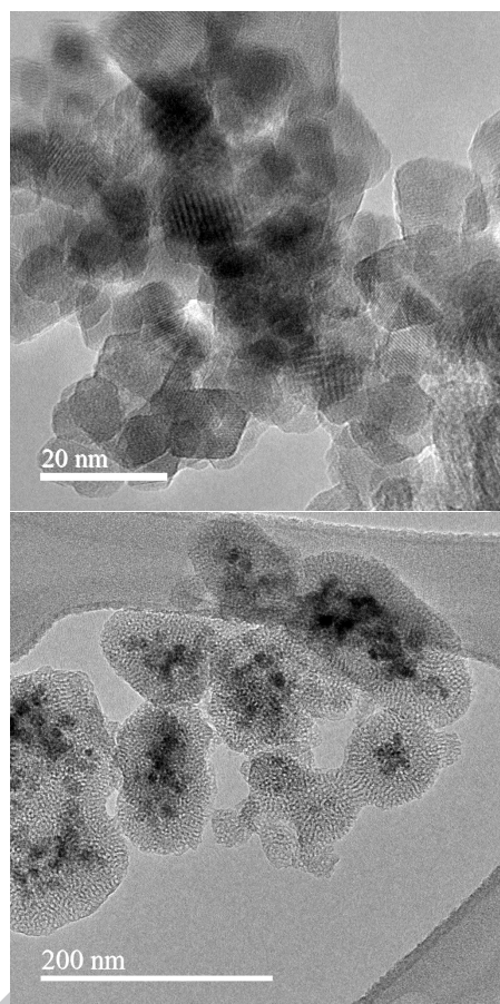
Figure 2. HR-TEM for the core-only sample (top panel), consisting of spherical \gamma\text{-Fe}_2\text{O}_3 nanoparticles, and the multi-core-shell sample (bottom panel) consisting of multiple \gamma\text{-Fe}_2\text{O}_3 nanoparticles as the core and silica as the shell. The images have different scales.
