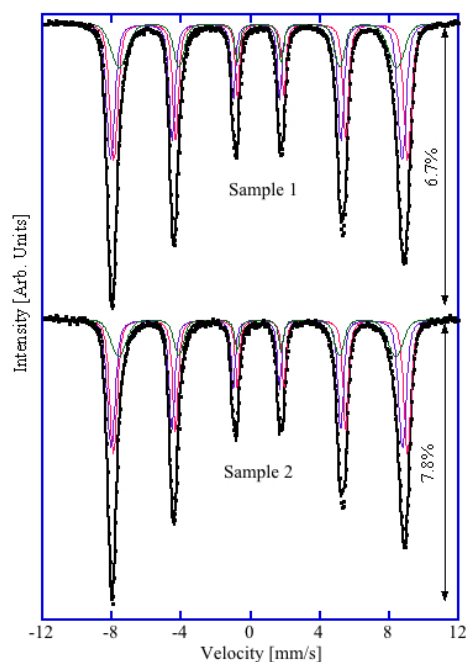
Figure 4. (Color online) Mössbauer spectra for both samples measured at 10 K.
