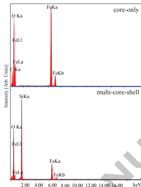
Figure 3. (Color online) EDXS for the core-only sample (top panel) and the multi-core-shell sample (bottom panel). The incorporation of \text{SiO}_2 is clearly seen in the multi-core-shell sample.
