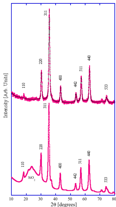
Figure 1. (Color online) XRD for the core-only sample (top panel), with the red dots as the experimental data and the solid black line as the fit, and the multi-core-shell sample (bottom panel). The diffraction peaks show clearly that the magnetic core consists of nanoparticles with inverse spinel structure. The broad peak around 24^\circ in the XRD for the multi-core-shell sample (bottom panel), as indicated in the figure, is from the \text{SiO}_2 .
