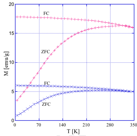
Figure 6. (Color online) ZFC and FC measurements in the temperature interval of 5–350 K in an applied field of 100 Oe for the core-only sample (+) and for the multi-core-shell sample (×).
