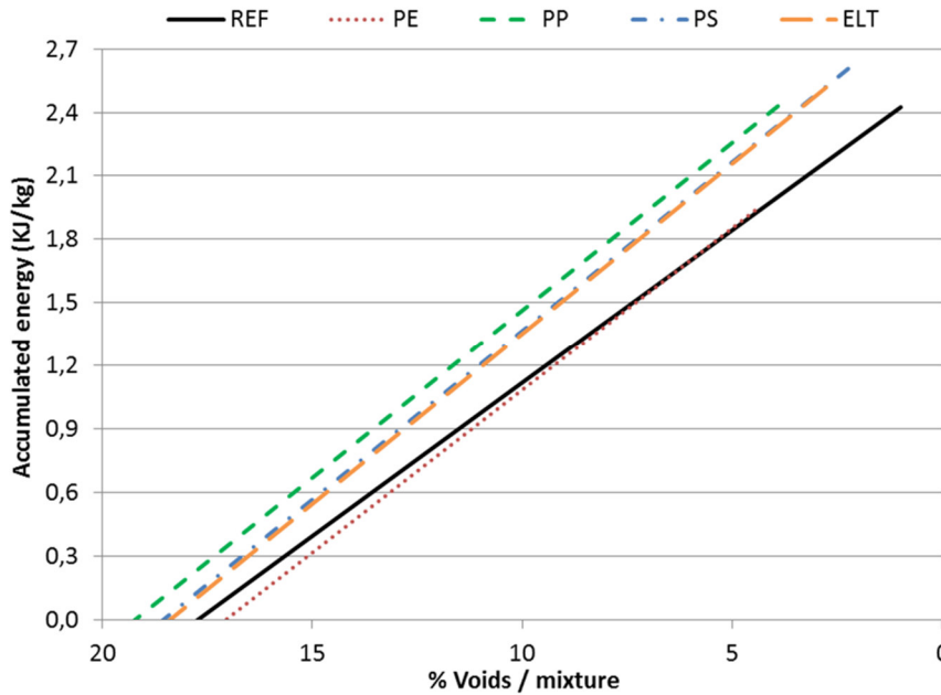
Figure 11. Energy of compaction - Voids
