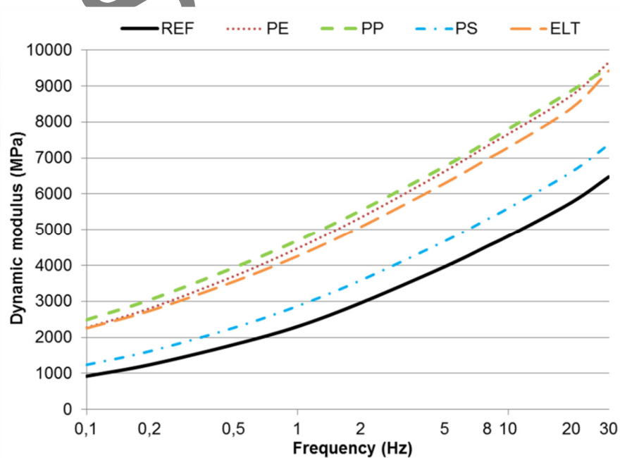
Figure 6. Dynamic stiffness of each type of mixture
