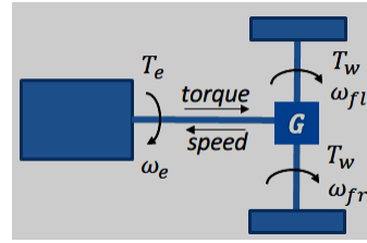
Figure 6. Transmission model.
