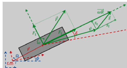
Figure 4. Geometric model of the tires.
