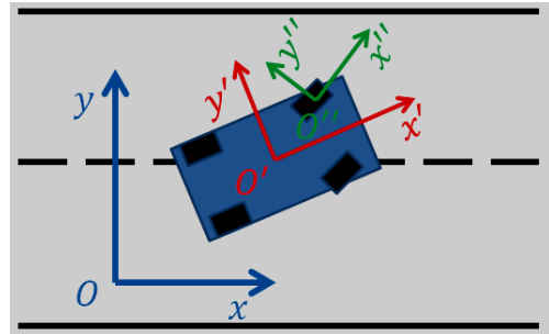
Figure 3. Reference frames.
