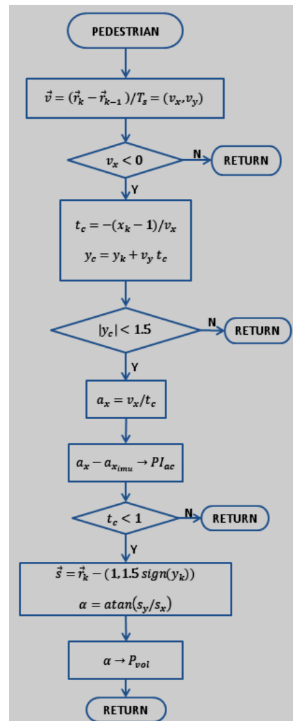
Figure 11. A flow chart showing the control algorithm.
