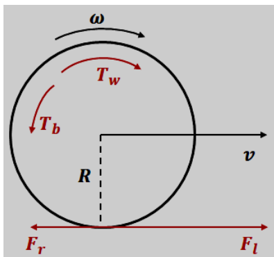
Figure 5. Wheel dynamics.
