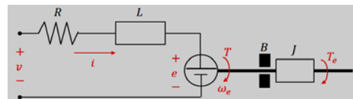
Figure 7. Electric motor.
