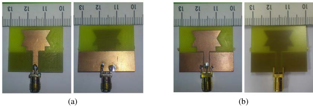
Figure 3. Fabricated antenna fed by: (a) microstrip line and (b) CPW.
