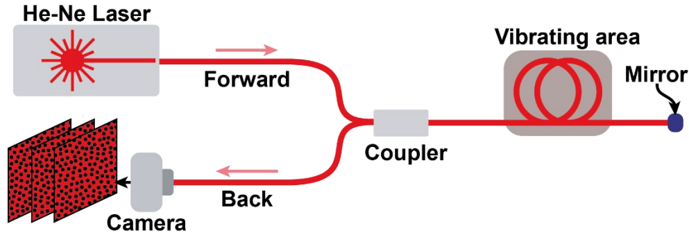
Figure 1. Experimental setup: A HeNe laser is launched through a 50:50 coupler to a multimode fiber whose free end is mirrored using a metallic surface. Light reflected at the end of the fiber travels back up to the detecting camera that records the specklegram sequence while a small fiber portion is under perturbation.
