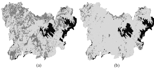
Fig. 11. Coverage maps in Ourense. The covered, not covered and filtered locations are depicted in light gray, dark gray and black, respectively. (a) Initial. (b) Optimized, but switching off all transmitters sector antennas in the range [-20, -15] dB.
