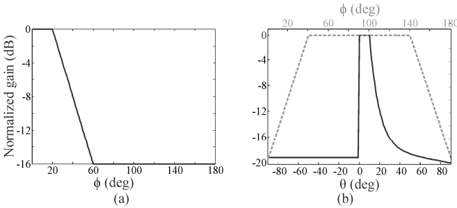
Fig. 2. (a) Terrestrial receiver antennas, detail of the azimuth radiation pattern. (b) Transmitter sector antennas, detail of the azimuth and elevation radiation pattern.
