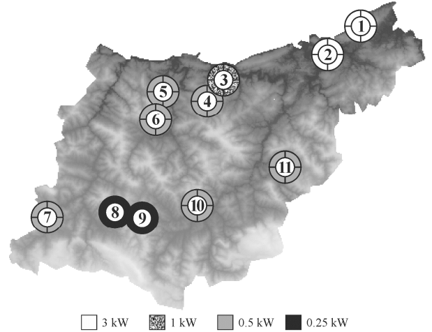
Fig. 4. SFN in Gipuzkoa. Initial transmission powers.
