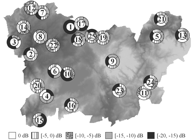
Fig. 8. The SFN in Ourense. Detail of sector antennas gain and their relative orientations in azimuth provided by one single run of the SA algorithm considering the ITU-R P.1812 and the k-LNM method.
