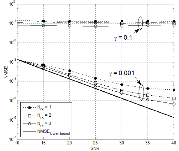
Fig. 3: NMSE performance in function of N_{\text{rx}} ( N_A = 4, N_B = 6, N_E = 5 ).
