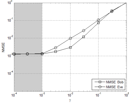
Fig. 4: NMSE performance in function of \gamma for N_A = 4 , N_B = 6 , N_E = 5 , \text{SNR} = 10\text{dB}
