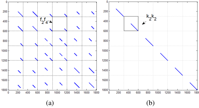
Fig. 2: Structure of covariance matrices. Example with N_A = 4, N_B = 6, N_E = 5, N_{\text{rx}} = 2, T_0 = T_1 = 150 (a) Matrix \mathbf{C}_{ff} , (b) Matrix \mathbf{C}_{kk}
