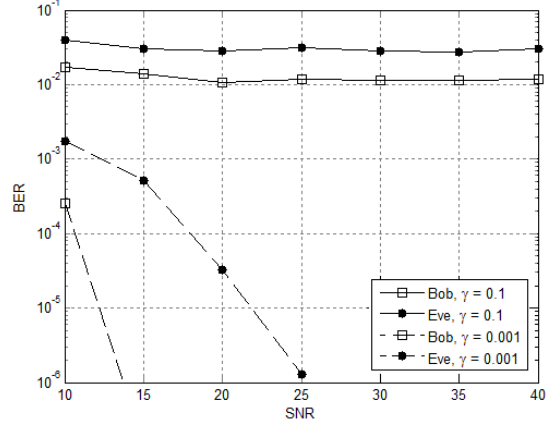
Fig. 5: BER performance in function of SNR for N_A = 4 , N_B = 6 , N_E = 5
