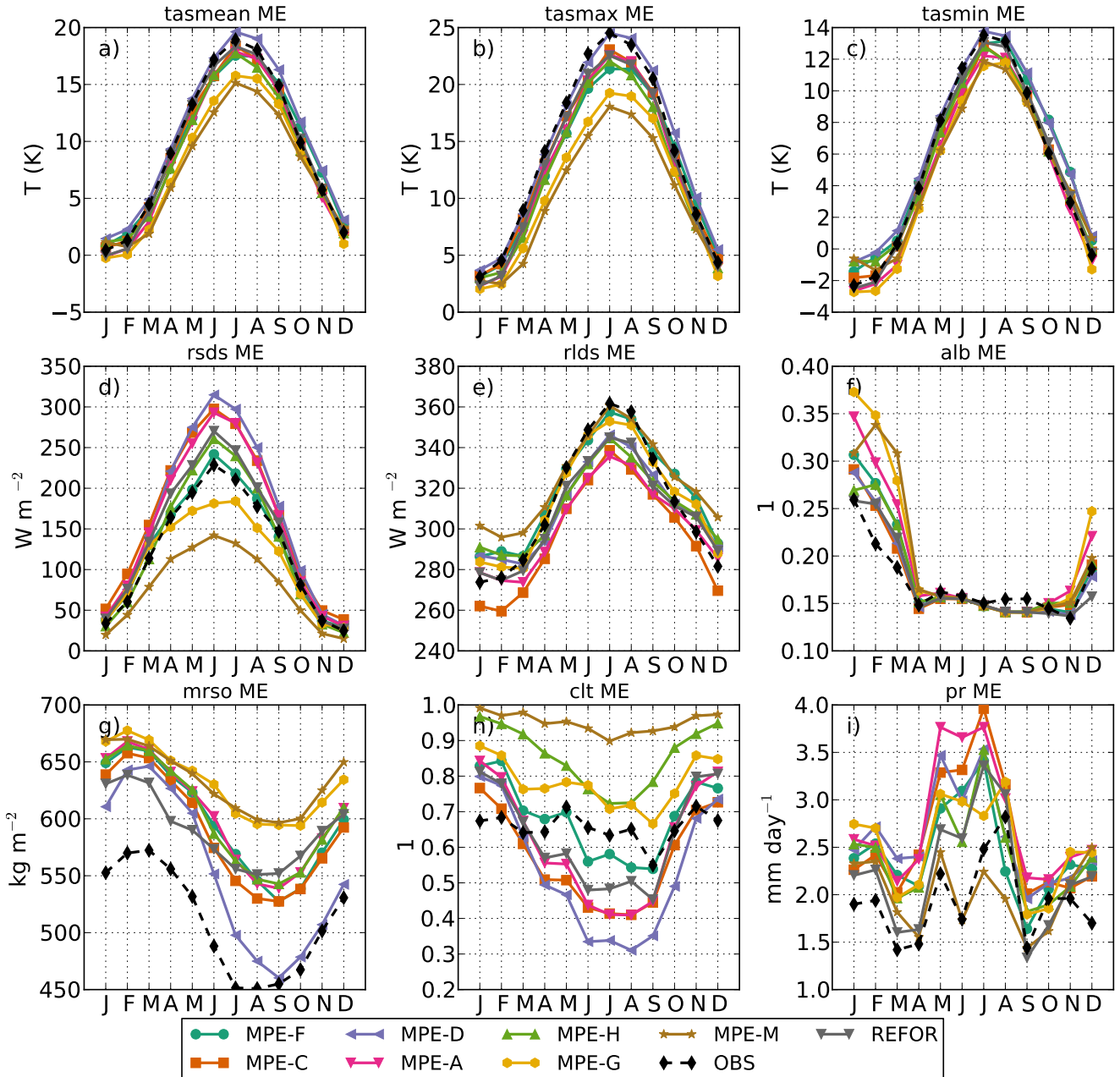
Fig. 12 Mean annual cycles of areal averages over the Middle Europe PRUDENCE region. The variables plotted are TASMEAN, TASMIX, RSDS, RLDS, MRSO, ALB, CLT and PR.
