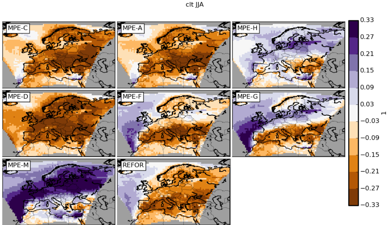
Fig. 6 Bias for total cloud cover in JJA respect to CERES-SYNdef1. The areas with no observed data are painted grey.
