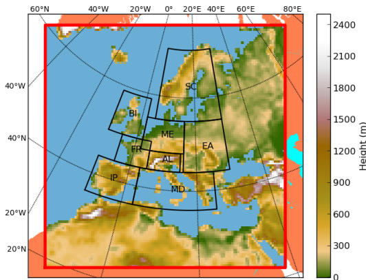
Fig. 1 Model domain and topography
