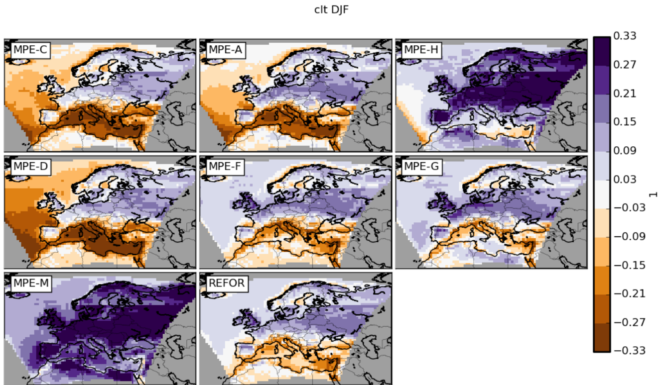
Fig. 9 Relative bias for CLT in DJF respect to CERES SYndef1. The areas with no observed data are painted grey. Note that the data are problematic above 60° latitude.
