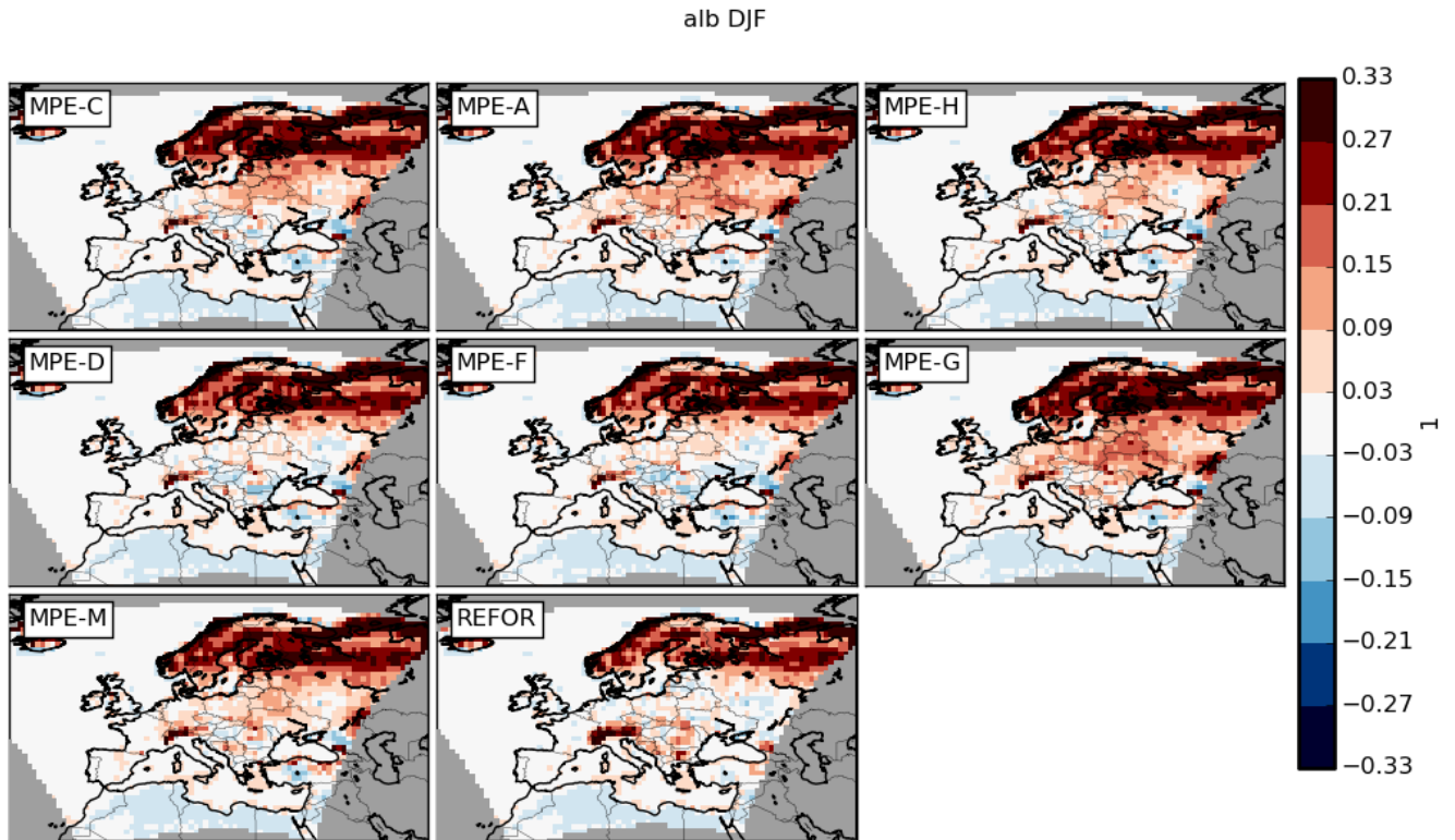
Fig. 10 Surface albedo bias in DJF respect to CERES EBAF. The areas with no observed data are painted grey. Note that the data are problematic above 60° latitude.
