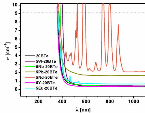
FIGURE 3. Absorption spectra ( \alpha vs \lambda ) of borotellurite glasses.
