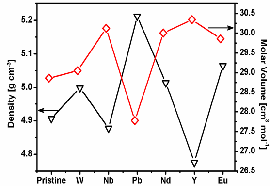
FIGURE 2. Density and molar volume variation in borotellurite glasses containing metal oxides.
