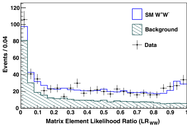
FIG. 1 (color online). The \text{LR}_{WW} distributions for the signal ( W^+W^- ) and background processes after a maximum-likelihood fit to the data.
