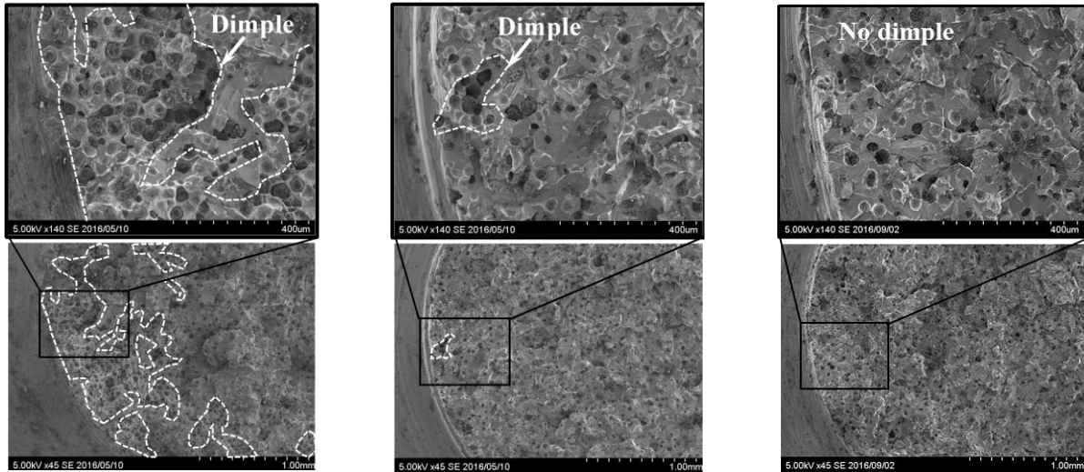
(a) Fracture surface at plot A in Fig.10 (b) Fracture surface at plot B in Fig.10 (b) (c) Fracture surface at plot C in Fig.10 (b) ( R = 5969 \text{ K} , \sigma_B^{\text{notch}} = 836 \text{ MPa} ) ( R = 5048 \text{ K} , \sigma_B^{\text{notch}} = 876 \text{ MPa} ) ( R = 3943 \text{ K} , \sigma_B^{\text{notch}} = 776 \text{ MPa} )
