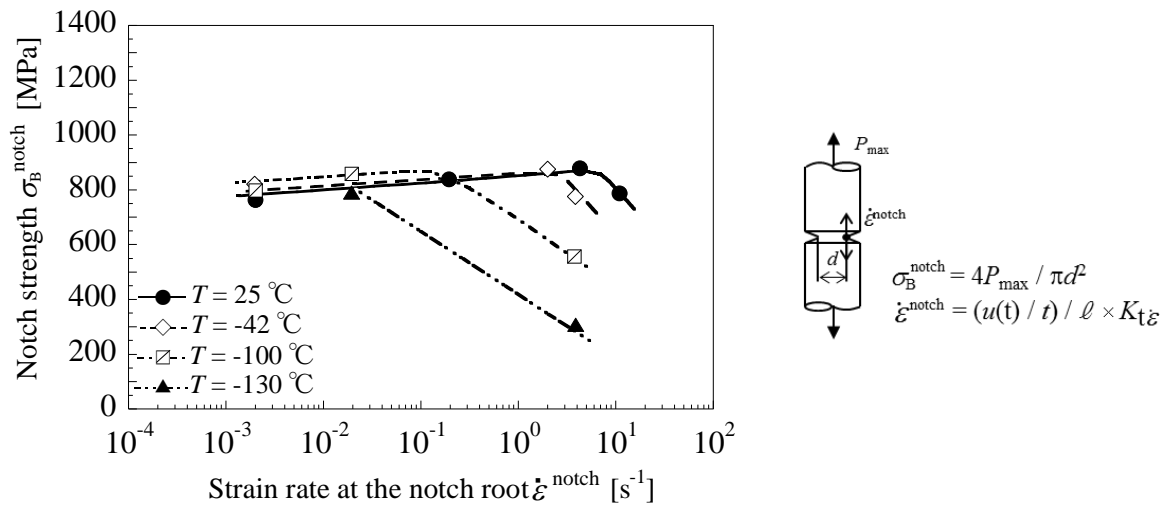
Fig. 7 Relationship between notch strength \sigma_B^{\text{notch}} ( \rho = 0.25 \text{ mm} ) and strain rate at the notch root \dot{\epsilon}^{\text{notch}} in the temperature range of -130 \sim 25 \text{ }^\circ\text{C} . Strain rate dependence of \sigma_B^{\text{notch}} is influenced by the test temperature.
