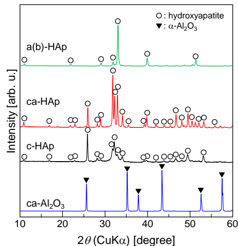
22 23 24 25 26 27 28 29 30 31 32 33 34 35 36 37 38 Figure 1. XRD patterns of samples a(b)-HAp, ca-HAp, c-HAp and ca- \text{Al}_2\text{O}_3 .
