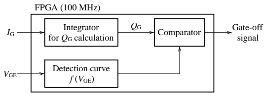
Fig. 5. Block scheme of FPGA.
