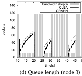
Fig. 6. Bottleneck node is switching node or upstream node (The bandwidth of Channel 2 set at 20 to 60 Mb/s)
