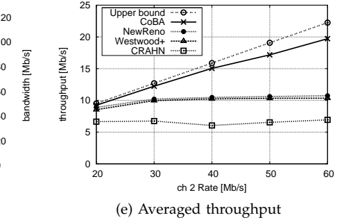
Fig. 6. Bottleneck node is switching node or upstream node (The bandwidth of Channel 2 set at 20 to 60 Mb/s)
