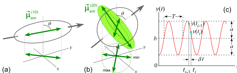
Fig. 2. Conceptual detection schemes for (a) linearly-polarized emission by a linear emitting transition dipole and (b) plane-polarized emission from a twofold degenerate dipole. Sample xy -plane is indicated. The graph in (c) indicates the time-trace pattern expected to be obtained by polarization modulations and the figure includes some of the parameters used in the following analysis..
