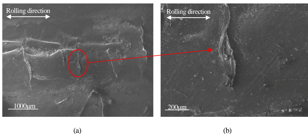
Fig. 15 Damaged plastic film B observed by SEM at the support pipe side surface after rolled 300 cycles when P=75N , T=70^{\circ}C and d_1=d_2=38mm . (a) Line scar of plastic film B observed from inside. (b) Detail of the line scars.
