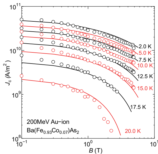
Fig. 1. Magnetic field dependence of critical current density in irradiated Ba-122 at various temperatures. Solid lines represent the theoretical value by the flux creep-flow model.
