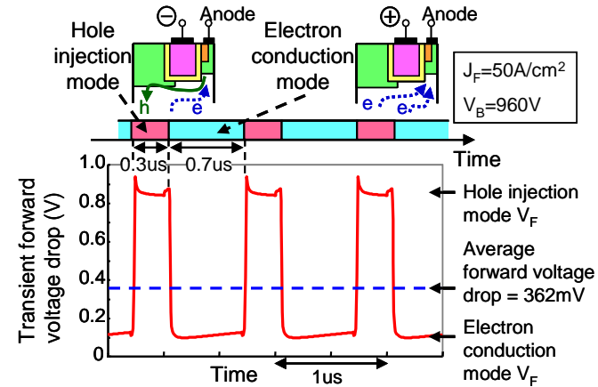
Figure 3. The transient forward voltage drop of the proposed diode at 1MHz pulse frequency at 50A/cm 2 . The average forward voltage drop is as low as 362mV for this case.
