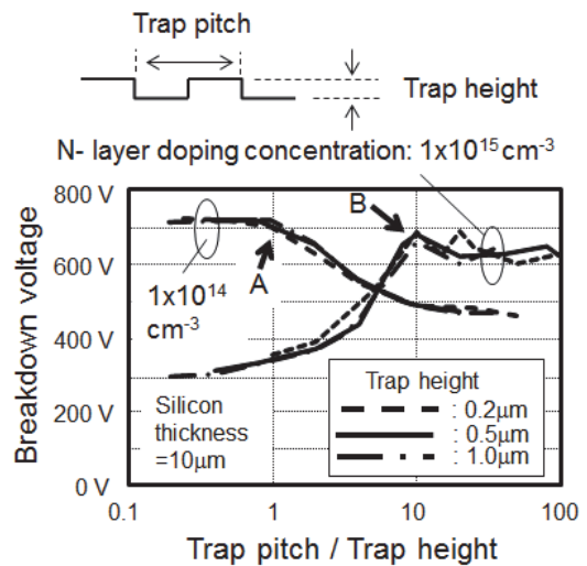
(a) Breakdown voltage change with trap design
