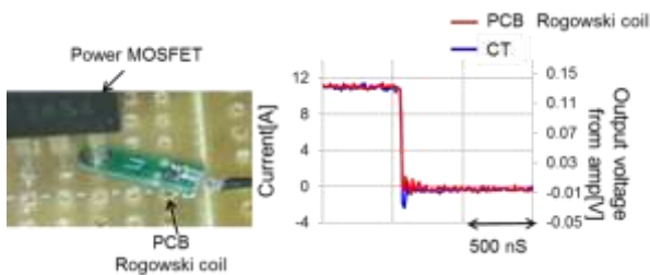
Figure 16 Demonstration with a very small Rogowski coil
