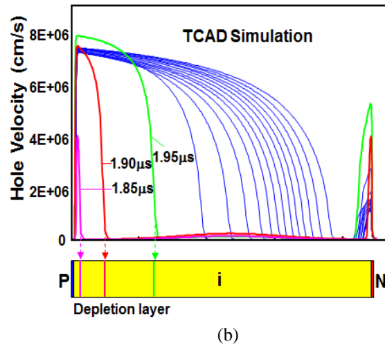
Fig.7. Increase in peak collector current (a) the time change of hole density and hole velocity in PiN diode (b).
