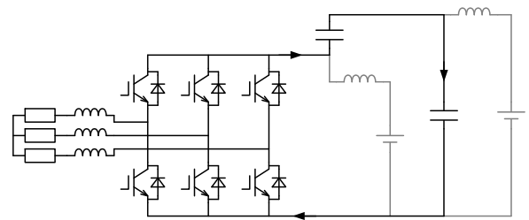
Fig. 3 New evaluation circuit using a three-phase voltage-source inverter (VSI).
