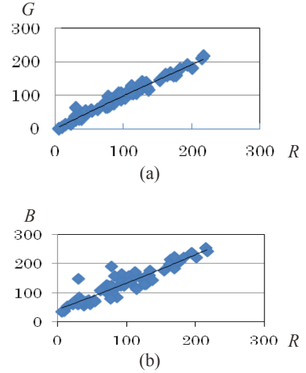
Fig. 5 The RGB relations with respect to the blue of the roof-top mark: (a) R - G relation, (b) R - B relation.
