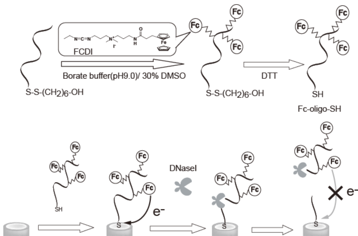
Fig. 1. Principle of electrochemical DNase I assay based on Fc-oligo-SH -immobilized electrode and chemical structure of FCDI .
