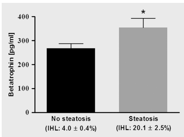
► Fig. 3 Associations of ANGPTL8/betatrophin with hepatic steatosis in the B-SMART cohort. Stratification according to IHL revealed that subjects with hepatic steatosis (20.1 ± 2.5% IHL, n = 15) had elevated ANGPTL8/betatrophin compared to nonsteatotic (4.0 ± 0.4% IHL, n = 42) subjects (p = 0.033). Data are shown as mean ± SEM; IHL, intrahepatic lipids; * p < 0.05.
