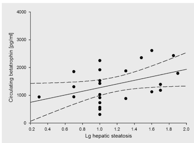
► Fig. 2 Association of circulating ANGPTL8/betatrophin with hepatic steatosis in INSIGHT subjects. Scatter plots illustrate correlation of circulating ANGPTL8/betatrophin with logarithmized liver steatosis ( r = 0.42 , p = 0.047 ). Lines indicate the 95% confidence intervals.
