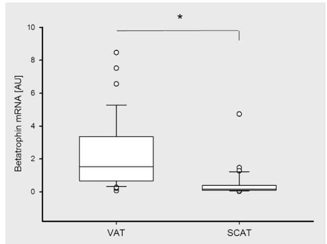
▶ Fig. 1 ANGPTL8/betatrophin mRNA in subcutaneous vs. visceral adipose tissue. ANGPTL8/betatrophin mRNA was detectable in 92% of VAT samples in INSIGHT study subjects and 75% SCAT samples. Levels of ANGPTL8/betatrophin mRNA were significantly increased in human VAT compared to SCAT (p < 0.001). SCAT: Subcutaneous adipose tissue; VAT: Visceral adipose tissue. Boxes span from 25 th –75 th percentile, error bars indicate 10 th and 90 th percentile; * p < 0.05.
