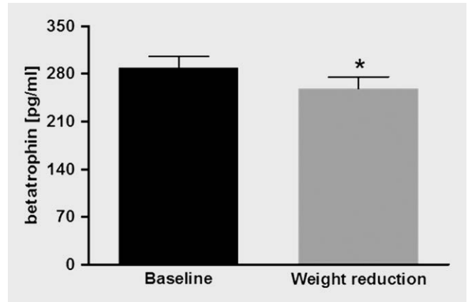
► Fig. 4 Association of ANGPTL8/betatrophin with weight loss in B-SMART. After a mean weight loss of 6.9 kg (= 7.4% initial body weight) due to dietary intervention accompanied by a 45% IHL reduction, ANGPTL8/betatrophin decreased by 11% (p = 0.015). Data are shown as mean ± SEM; IHL: Intrahepatic lipids; * p < 0.05.
