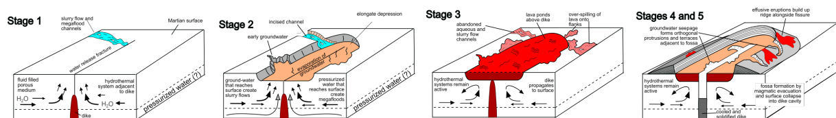
Figure 1. Proposed formation mechanism for Cerberus Fossae. All processes shown require the presence of a subsurface dike and an ice-rich cryosphere that provided fluids mobilized in a hydrothermal system. Modified from Pendleton (2015).
