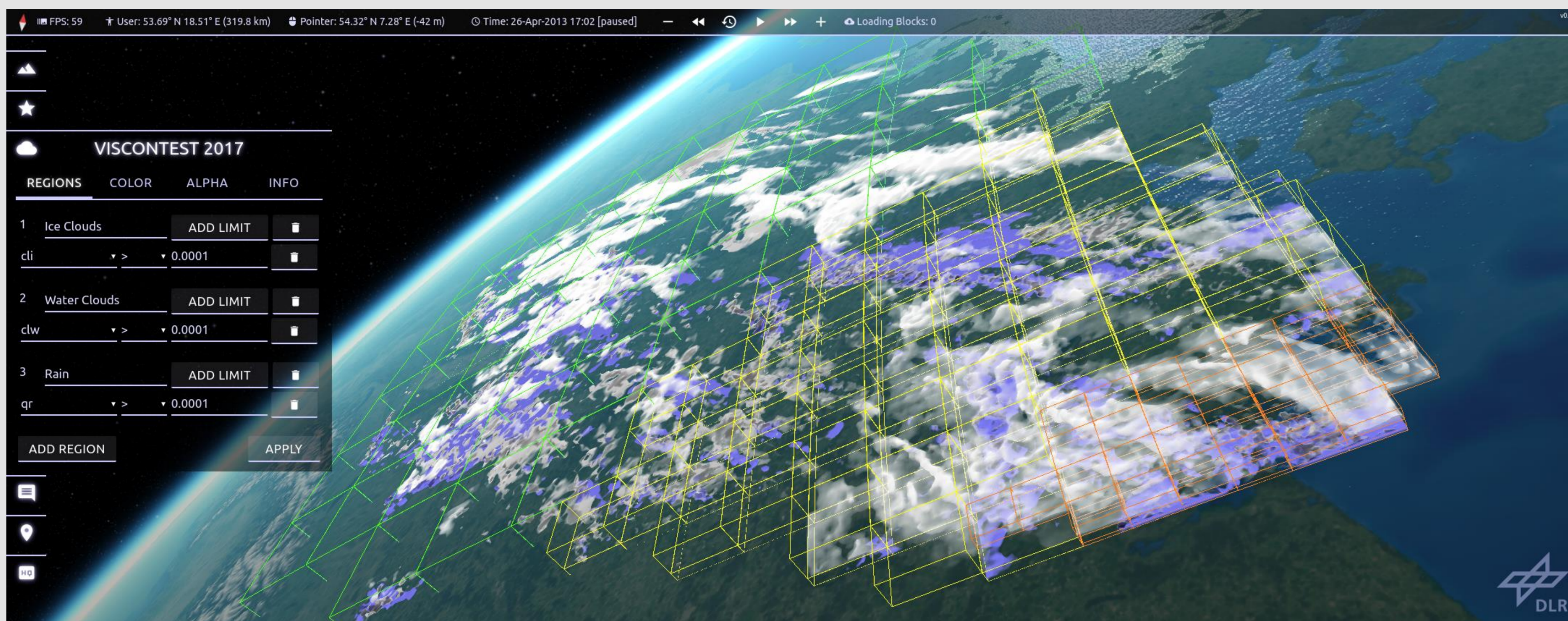
Real-time volumetric visualization of ice, water, and rain bands using our sub-volume selection mechanism in the graphical user interface. In addition, large terrain data is combined with the weather simulation to analyze their correlations.
