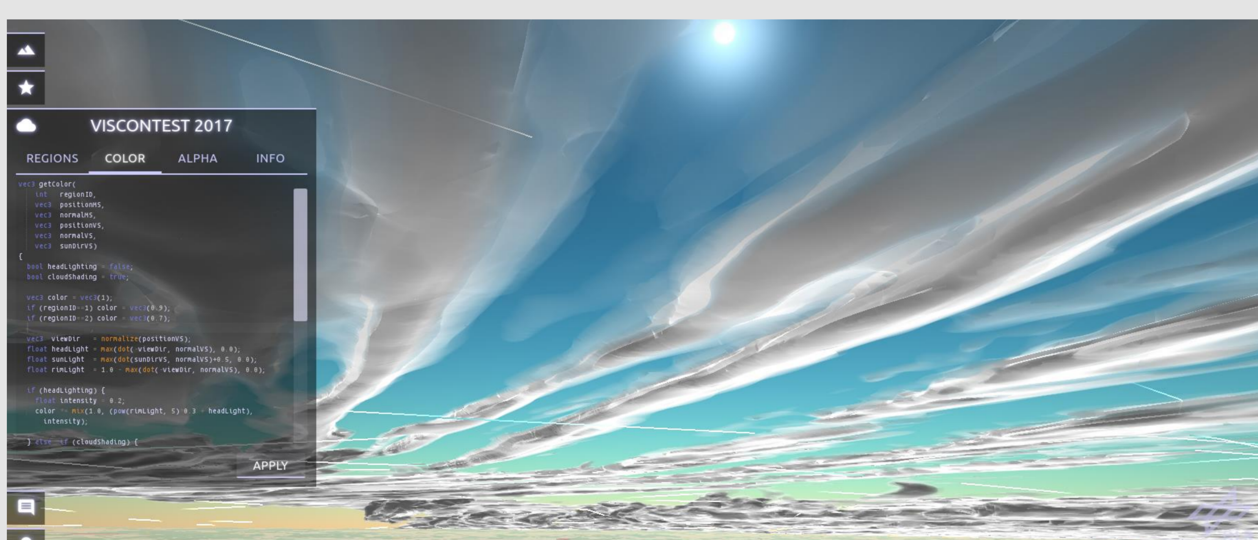
High altitude clouds in the southern part of the simulation domain. On the left hand side, the shader editor in the user interface can be seen. There are also some airplane trajectories visible in this image.
