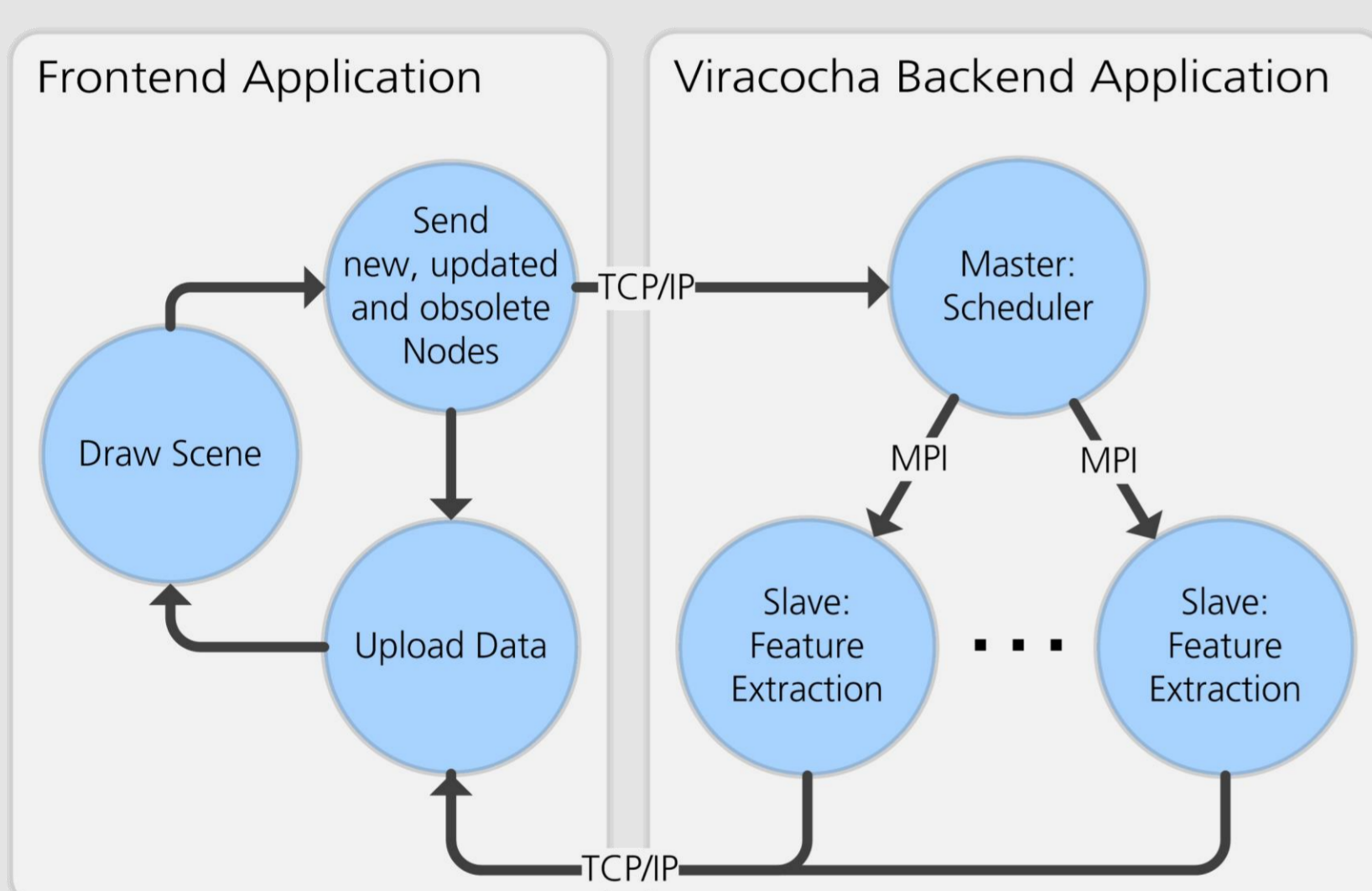
The rendering frontend selects nodes of the Level-of-Detail data structure for parallel processing. The backend executes the feature extraction on a cluster system and streams results back.
