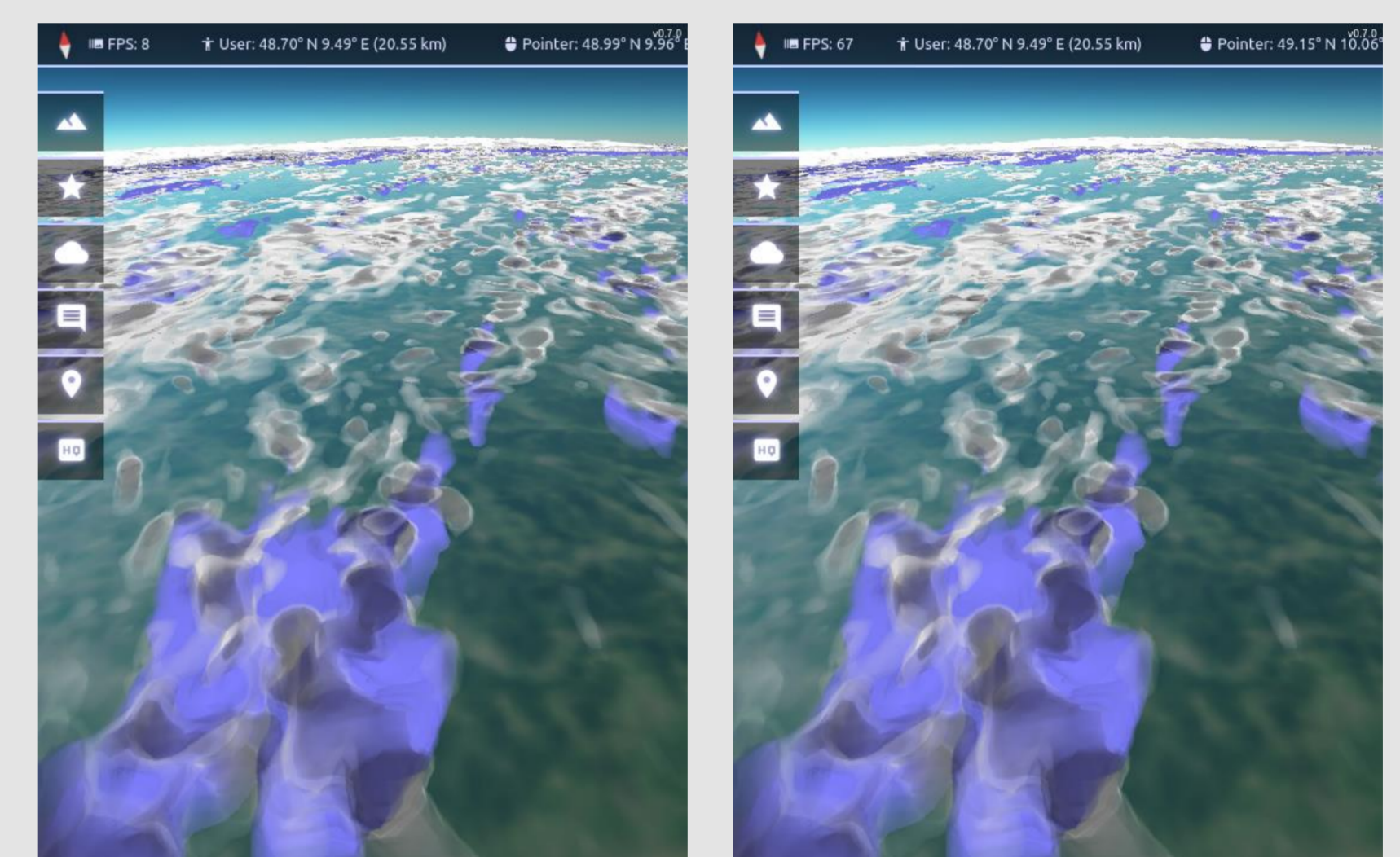
The full dataset cannot be rendered at interactive frame rates (left, 8 FPS). However, this is possible if a lower, view dependent resolution is used in the distance (right, 67 FPS). The error in is barely noticeable.
