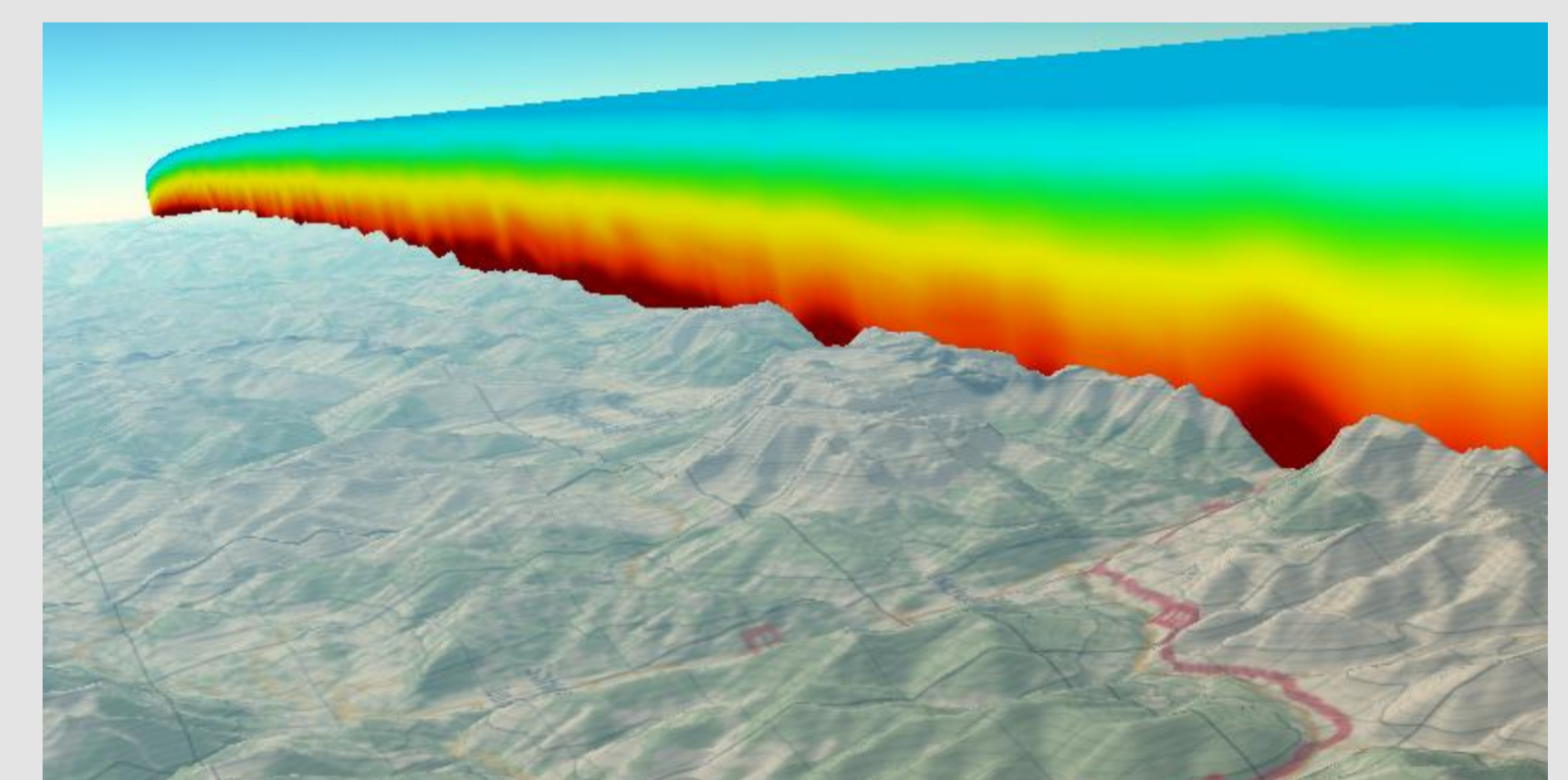
The southern border of the dataset with color-coded temperature based on SRTM30 digital elevation and Open Street Map data. The correlation between terrain and temperature distribution is apparent.
