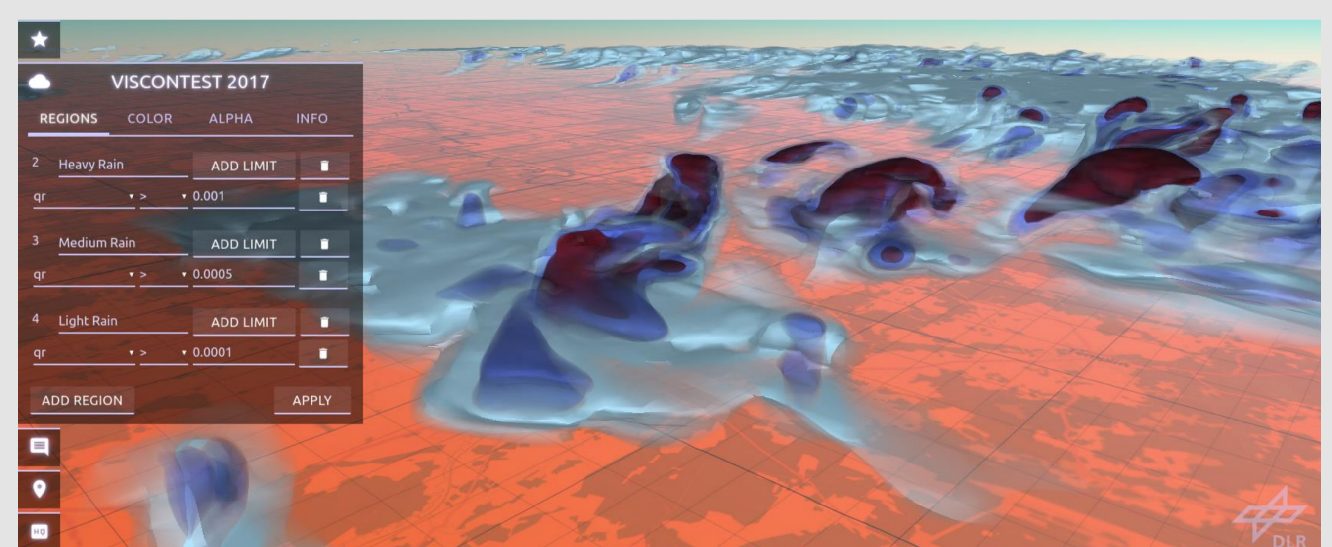
This is an example of intersecting volumes. Sub-volumes for three rain mixing ratios are inside each other. The pseudo-volumetric effect helps to understand the depth of the extracted regions.
