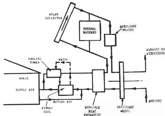
Fig. 4 'REVERS' Cycle
