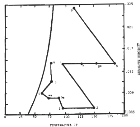
Fig. 5 'DINC' Cycle
