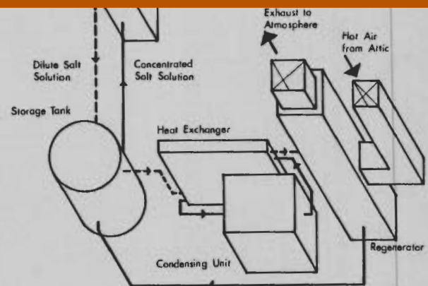
Figure 1. Overall Mechanical System
