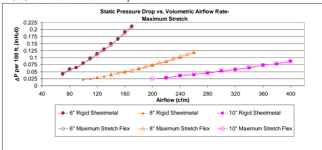
Fig.2. Static Pressure Loss in 6", 8", and 10" Non-Metallic Flexible Duct with Maximum Stretch Compared with Rigid Sheet Metal Duct
