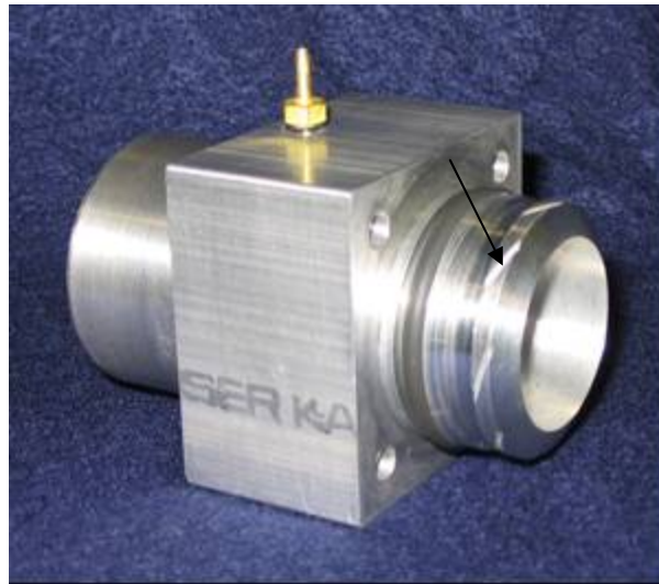
Figure 13. Outlet skimmer tested with shortened acrylic AAC. The arrow indicates one of eight grooves around the leading edge.
