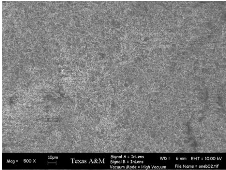
Figure 6. SEM photo of 1 bar rated ceramic surface.
