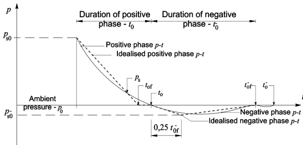
Figure 7 Pressure time history
