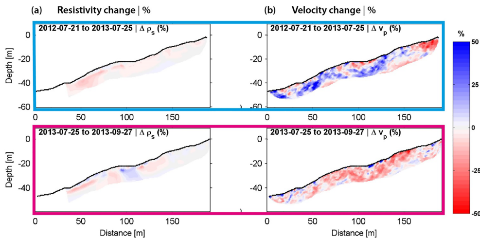
Figure 9. Temporal changes in (a) resistivity and (b) P-wave velocity between the measurements shown in Fig. 8. Upper panel: interannual changes between 21 July 2012 and 25 July 2013. Lower panel: seasonal changes between 25 July and 27 September 2013. The coloured rectangles correspond to the resistivity and velocity change patterns in the synthetic experiments (see Figs. 5–7).
