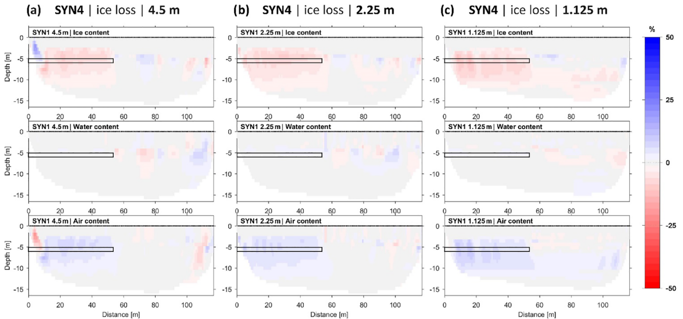
Figure 12. Comparison of 4PM-calculated changes in volumetric fractions for the inverted synthetic data of scenario SYN4 for three different sensor spacings: (a) 4.5 m, (b) 2.25 m, and (c) 1.125 m. The position of the introduced change is indicated by black lines.
