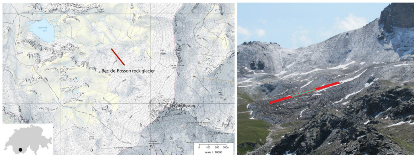
Figure 1. Map and photograph of the Becs de Bosson rock glacier. The red line on map and photograph marks the position of the full geophysical profile, while the green line on the photo shows the joint ERT/RST profile, which is used for the 4PM analysis of this study. Map source: Swiss Federal Office of Topography swisstopo.
