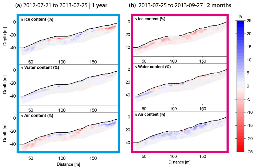
Figure 10. Changes in volumetric fractions for the two time intervals of inverted monitoring data of the Bees de Bosson rock glacier: (a) 1 year (July 2012 to July 2013) and (b) 2 months (July 2013 to September 2013). Note the reduced range of the colour scale.
