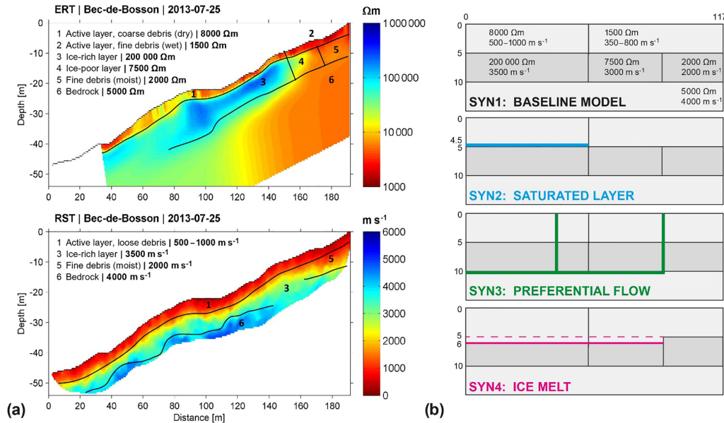
Figure 3. Creation of synthetic models based on inverted field data of the Becs de Bosson rock glacier: (a) inverted ERT and RST tomograms of 25 July 2013 with superposition of interpreted zones, (b) simplified synthetic baseline model (SYN1) based on the interpretation in (a) and different scenarios of hydrological processes (SYN2 to SYN4).
