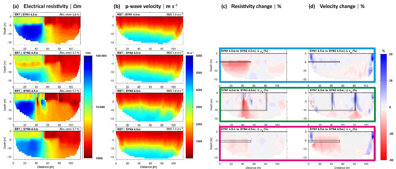
Figure 5. Inverted synthetic model sections of the synthetic model scenarios of Fig. 4 for (a) ERT and (b) RST, and percentage changes between (c) \rho_s and (d) v_p of the three scenarios with respect to the baseline model. The positions of the introduced changes between the different scenarios are indicated by black lines.
