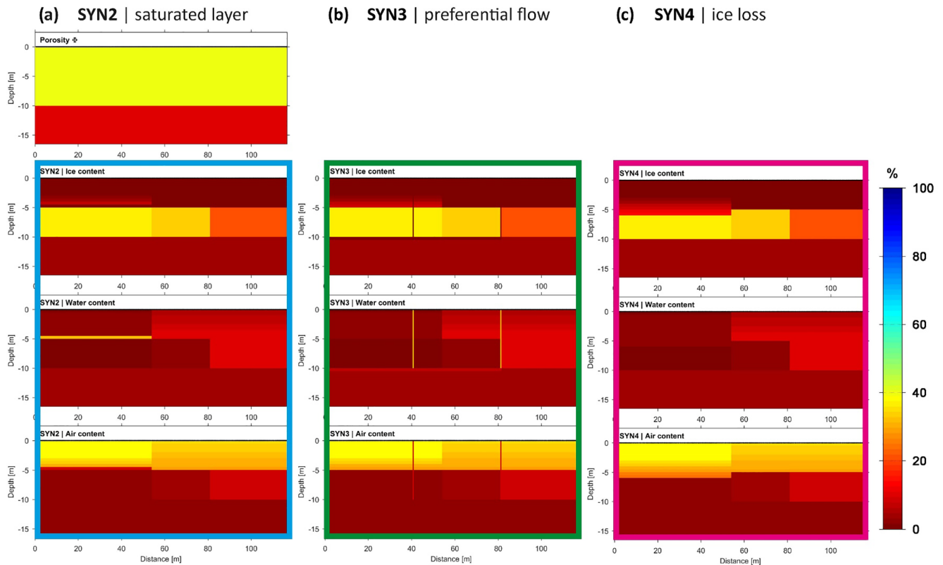
Figure 6. 4PM results for the synthetic model scenarios (see Fig. 4a, b). The blue, green and pink rectangles correspond to the same rectangles in Figs. 4, 5 and 7. The prescribed porosity model is shown in the uppermost panel.
