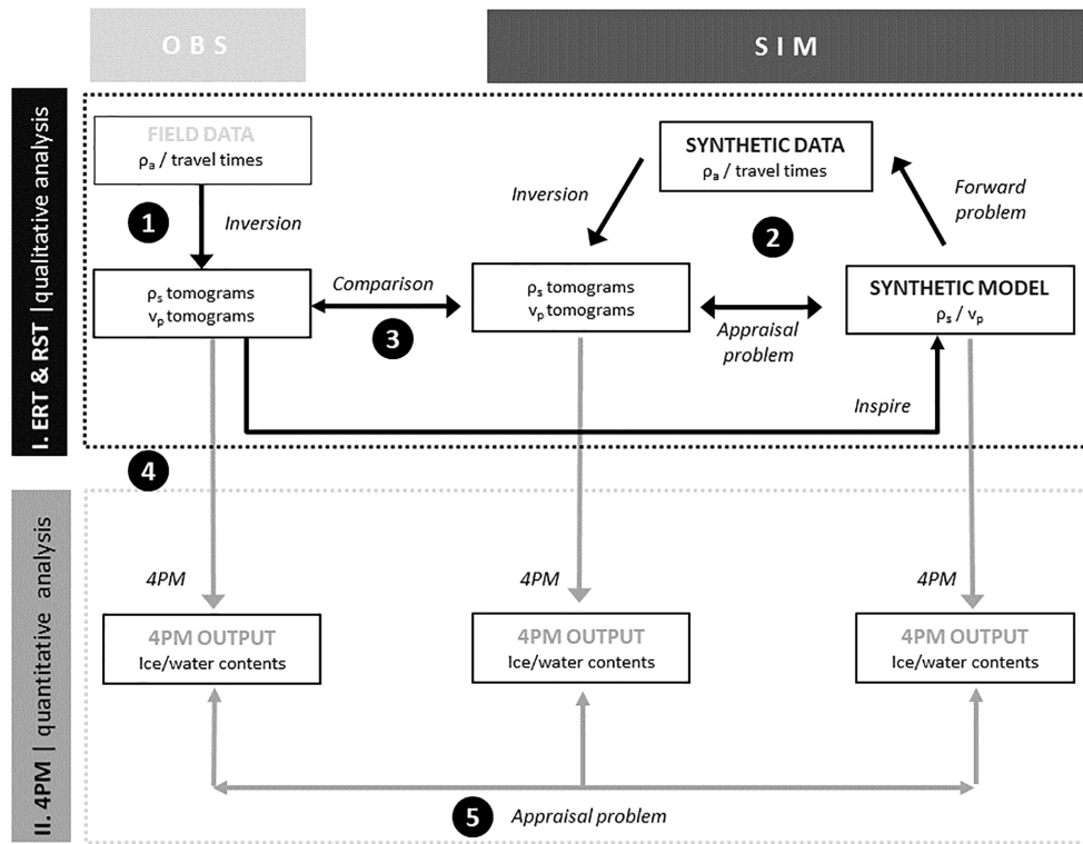
Figure 2. Overview of the work flow applied in this study. Here, \rho_a denotes the apparent resistivity, \rho_s the specific resistivity and v_p the P-wave velocity.
