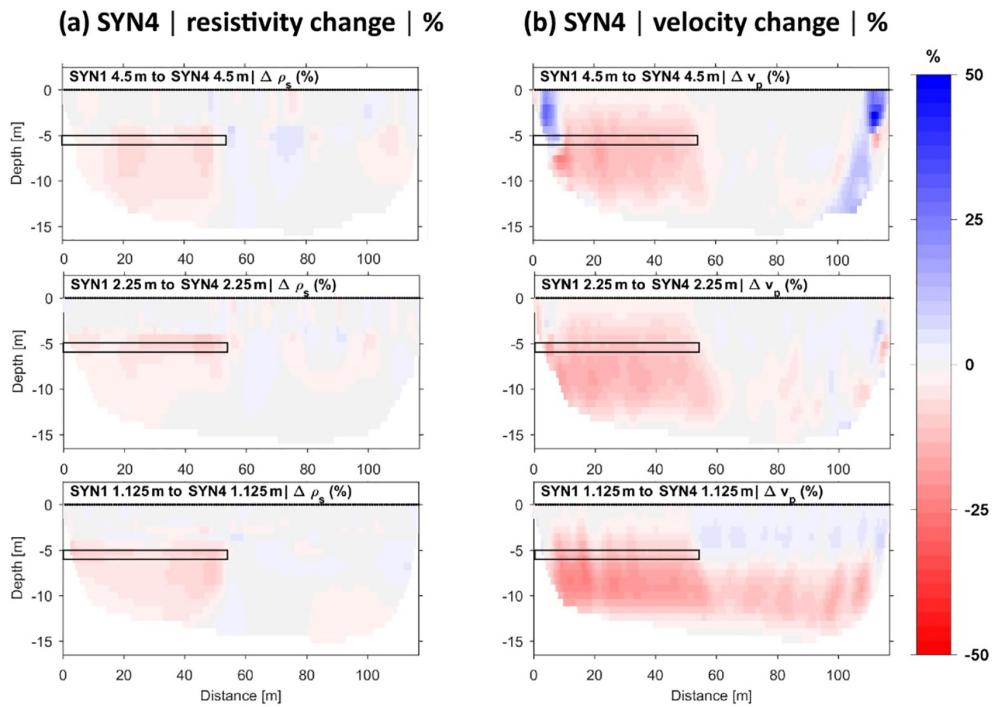
Figure 11. Comparison of (a) resistivity and (b) velocity changes of inverted tomograms for scenario SYN4 for three different sensor spacings. Top: 4.5 m, middle: 2.25 m, bottom: 1.125 m. The position of the introduced change is indicated by black lines.
