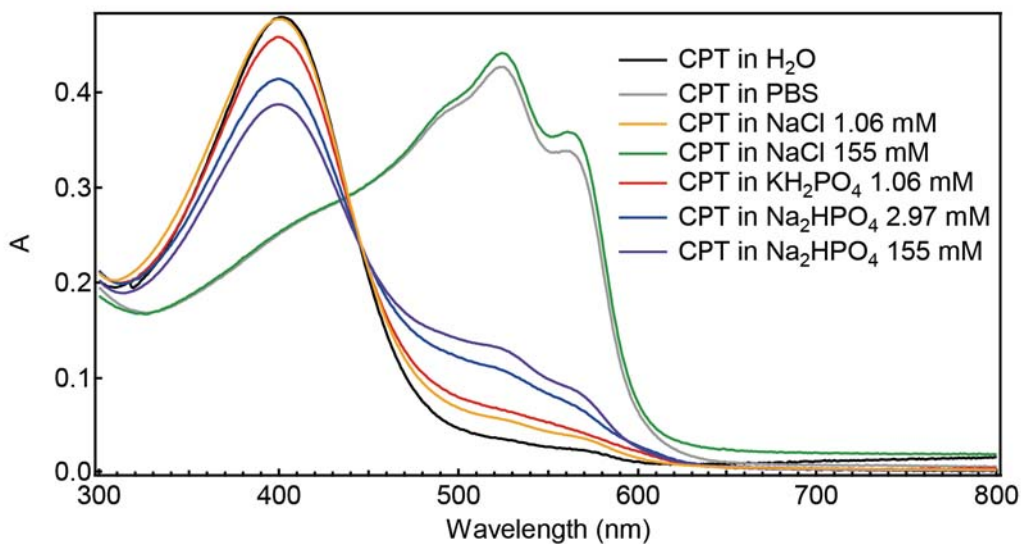
Figure S3 Absorption spectra of CPT ( 7.3 \cdot 10^{-5} M, monomeric basis) at 25^\circ\text{C} in water, in PBS and in different aqueous salt solutions.
