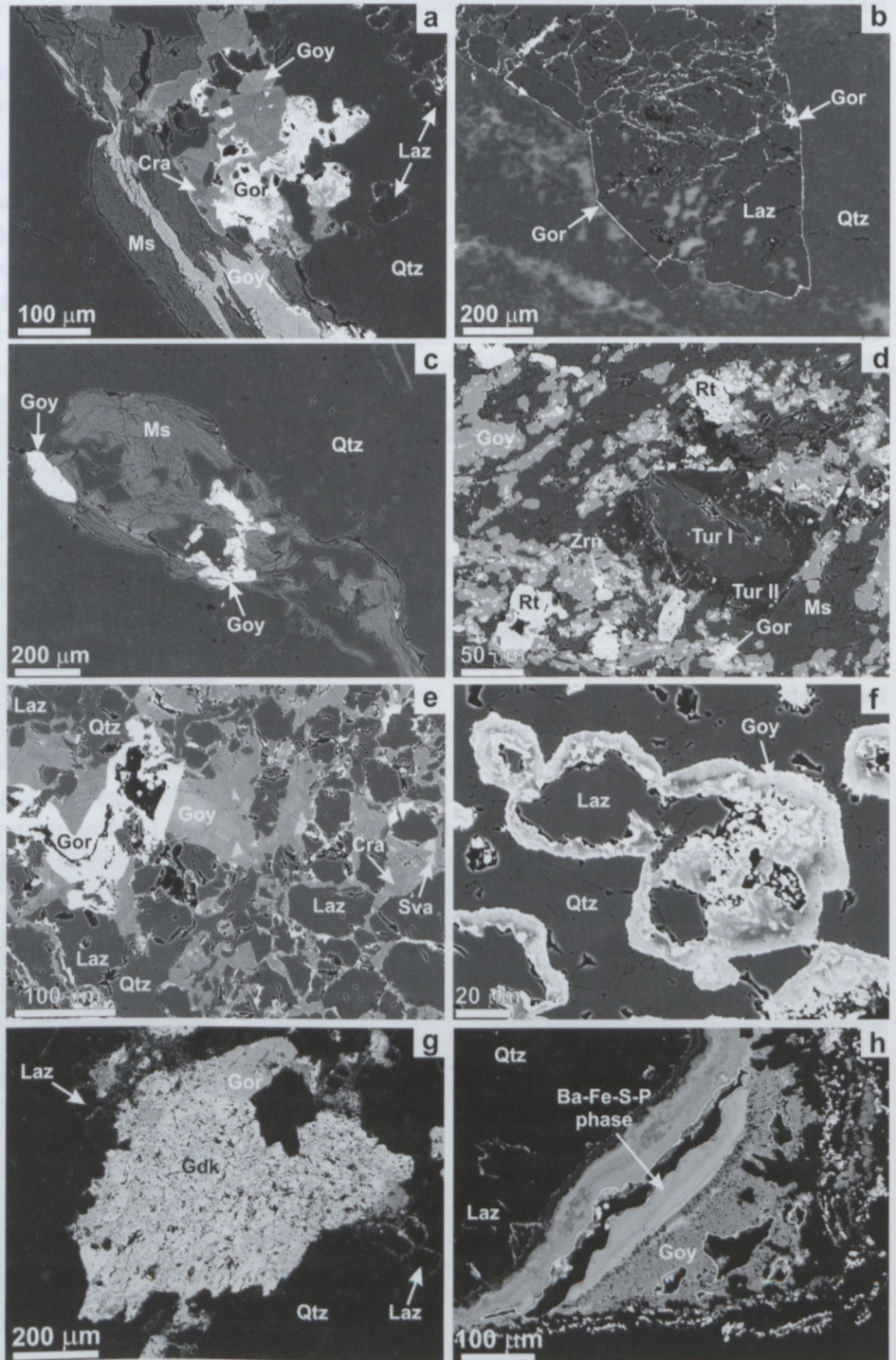
Fig. 5.4. BSE photomicrographs of lazulite (Laz) and associated gorceixite (Gor), goyazite (Goy), crandallite (Cra), svanbergite (Sva), goedkenite (Gdk), Ba-Fe-S-P-phase, muscovite (Ms), tourmaline (Tur), zircon (Zrn), rutile (Rt) in quartz (Qtz). Tribeč Mts. Photo: D. Ozdín.
