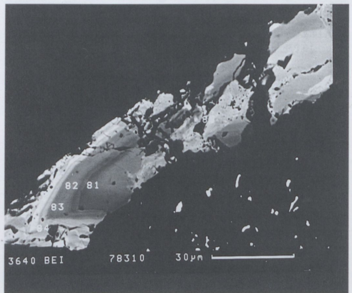
Fig. 14.6. Oscillation zoning of ferrocolumbite to manganocolumbite, Dlhá dolina valley. BSE image, photo: P. Sulovský.
