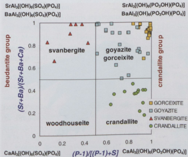
Fig. 5.6. Composition of (Ba,Sr,Ca) phosphates-sulphates from the Tribeč Mountains.
