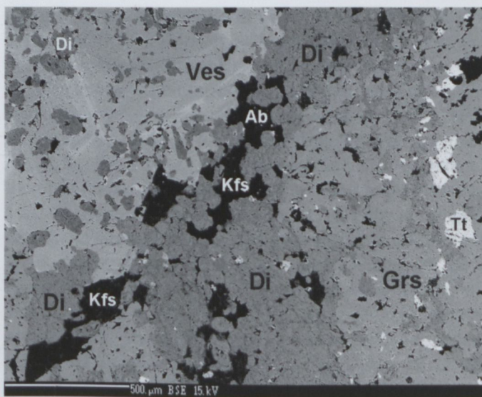
Fig. 4.3. Contact metamorphic assemblage of the Ca skarn, Dubová, Horné Trávniky. (Diopside (Di), vesuvianite (Ves), grossular (Grs), albite (Ab), K-feldspar (Kfs) and titanite (Tt). BSE micrograph, photo: D. Ozdín.
