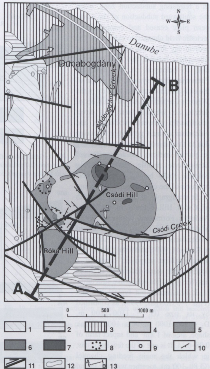
Fig. 6. Geological map of Csódi Hill and its surroundings, without Quaternary formations (Korpás, 1999). Legend: 1: Mátra Andesite Formation, 2: Budafok Formation, 3: Törökbálint Sandstone Formation, 4: Kiscell Clay Formation, 5: Amphibole-biotite dacite laccolith, 6: Crater, 7: Feeding channel, 8: Covered feeding channel, 9: Late feeding channel, 10: Dip of strata, 11: Fault and dextral fault, 12: Outcrop and observation point, 13: Geological section.
