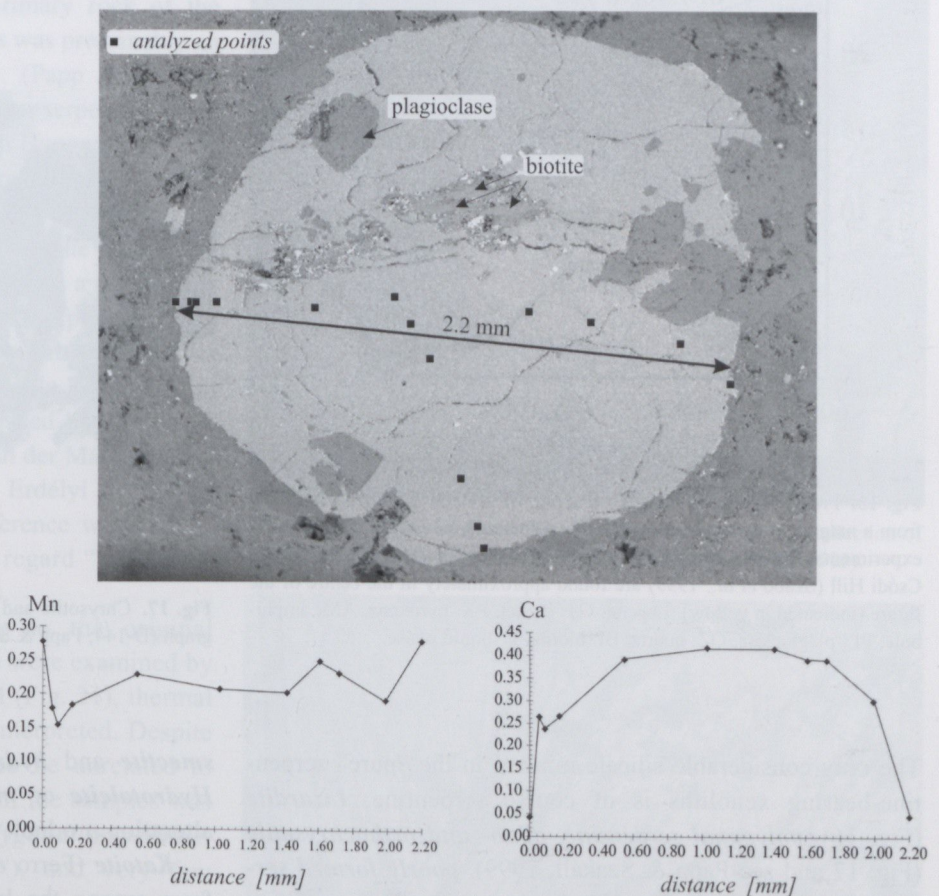
Fig. 13. Zoned almandine crystal (back scattered electron image, Szabó et al. , 1999). Dots indicate the microprobe measurements. Below: Distribution of Mn and Ca ( a.p.f.u. ) along the traverse marked on the figure.
