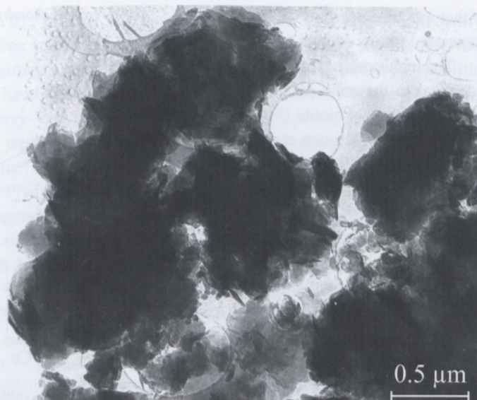
Fig. 16. Lizardite, xenomorphic flakes. TEM micrograph (D-139, Papp & Szakáll, 1999).
