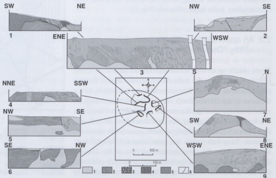
Fig. 8. The laccolith of Csódi Hill and its detailed sections as seen on the quarry walls (Korpás, 1999). Legend: 1: Area covered by soil and debris, 2: Fluidal banded dacite, 3: Blocky dacite, 4: Contact metamorphic clay, 5: Late feeding channels and breccias, 6: Fault.
