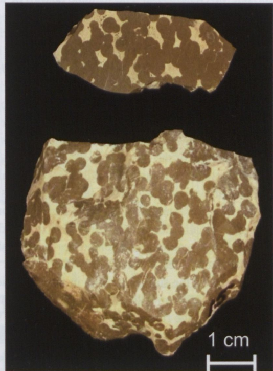
Fig. 5. Contact metamorphic spotted slate, hand specimen (below) and cut surface (above; photo: Orosz, E.), varieties with smaller spot size exist, too.
