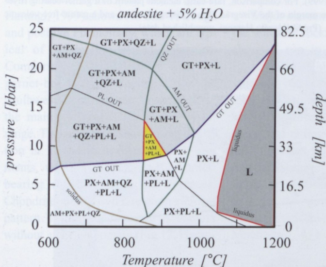
Fig. 15. Pressure-temperature (PT) diagram of mineral phases crystallizing from a magma of andesitic composition (containing 5 % H 2 O), based on the experimental data of Green (1982). The field of the coexisting minerals of the Csódi Hill (Szabó et al. , 1999) are found approximately in the centre of the figure (indicated in yellow). Legend: GT: garnet, PX: pyroxene, AM: amphibole, PL: plagioclase, QZ: quartz, BI: biotite, L: liquid phase.
