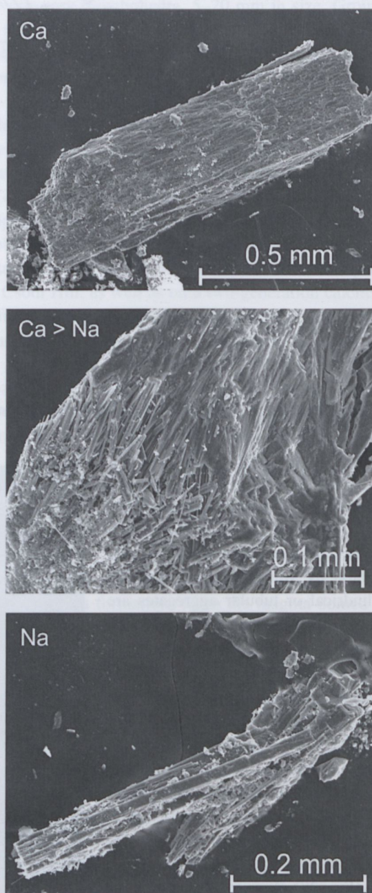
Fig. 29. SEM micrographs of the Csódi Hill acicular zeolite, grown on a crack surface of the contact spotted slate, together with analcime. The zeolite has natrolite structure (as proved by XPD), the dominant extra framework cation was most cases found to be Na (natrolite, lowermost image), but there were indications of Na-Ca mixed compositions (mesolite, middle image) and an almost pure Ca member (scolecite, uppermost image), too. Photographs and analyses taken by Melinda János.
