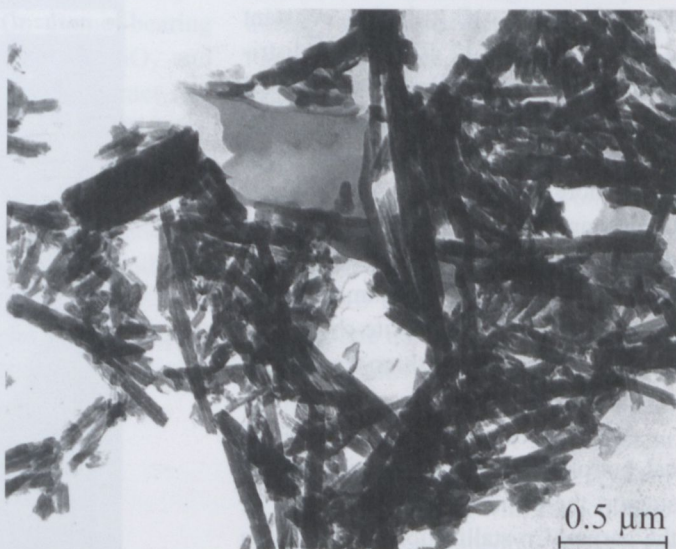
Fig. 17. Chrysotile and polygonal serpentine (thicker "rods"). TEM micrograph (D-144; Papp & Szakáll, 1999).
