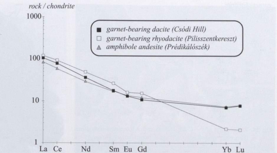
Fig. 12. Chondrite (Nakamura, 1974) normalised rare-earth element pattern of the garnet-bearing dacite from Csódi Hill (Harangi, 1999). For comparison, rare-earth element pattern of a garnet-bearing rhyodacite from the southwestern margin of the Visegrád Mts. (Pilisszentkereszt) and a garnet-free volcanic rock from the Visegrád Mts. (Prédikálószték; Harangi, unpublished data).
