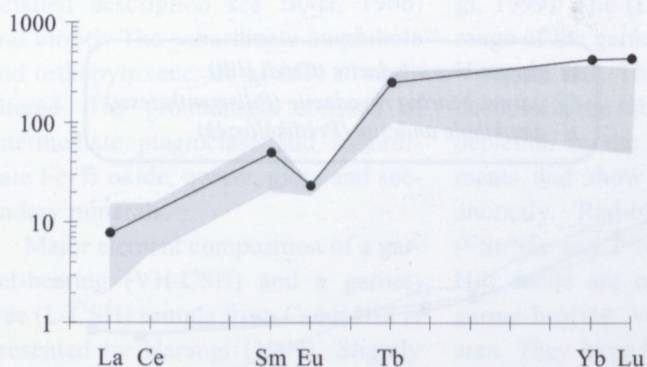
Fig. 14. REE content of the Csódi Hill almandine, compared with garnet samples from other calc-alkaline volcanites from Hungary (Kósa, 1998). Black dots: Csódi Hill almandine, grey band: area covered by the other garnets (Szabó et al. , 1999).
