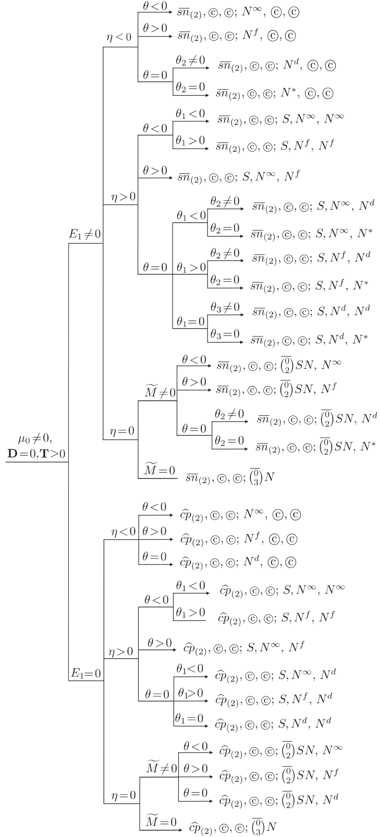
Diagram 1.1: Global configurations: the case \mu_0 \neq 0, \mathbf{D} = 0, \mathbf{T} > 0 .
