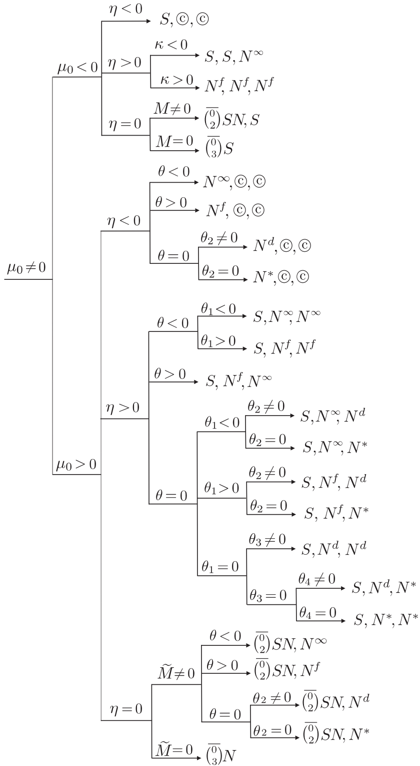
Diagram 3.1: Configurations of infinite singularities: the case \mu_0 \neq 0 .
