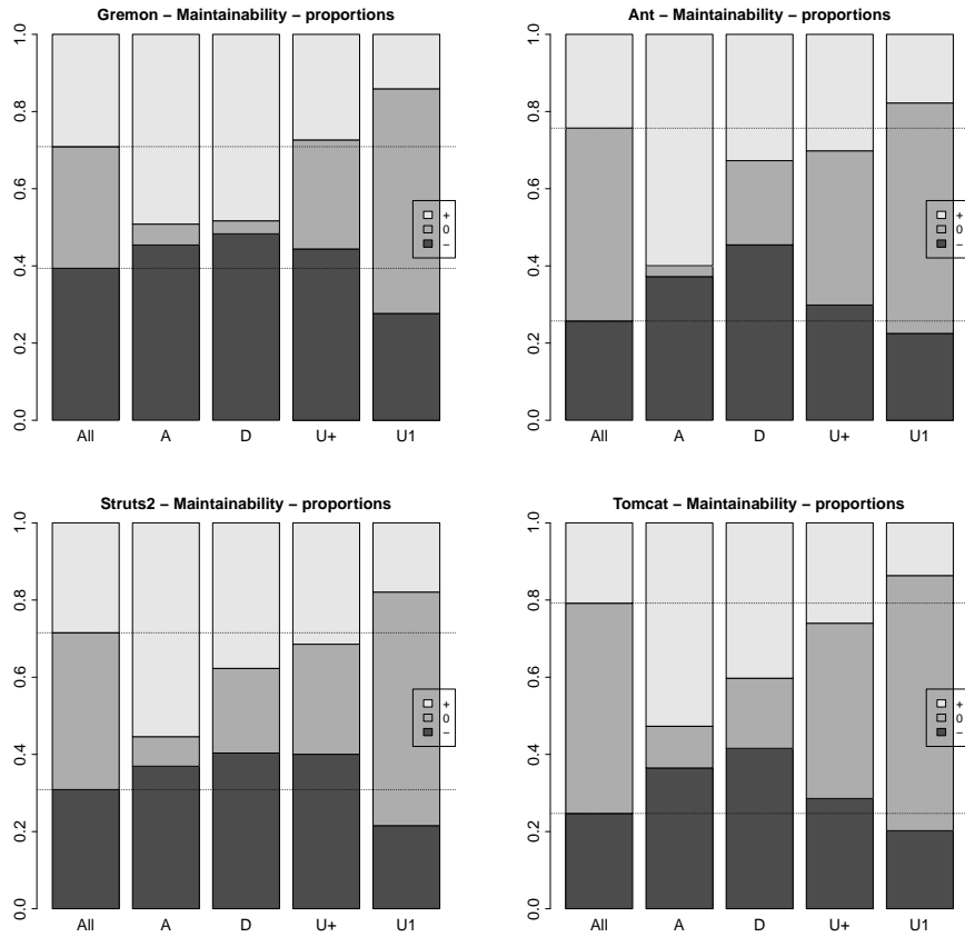
Figure 5: Maintainability proportions
