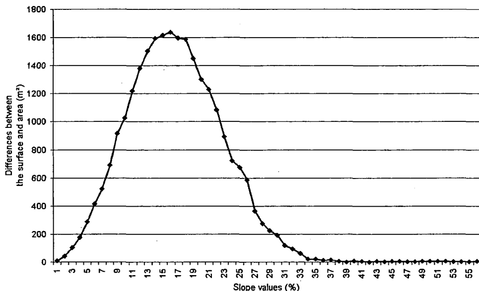
Fig. 4 The surface-addition graph of the slope values within the investigatid area
