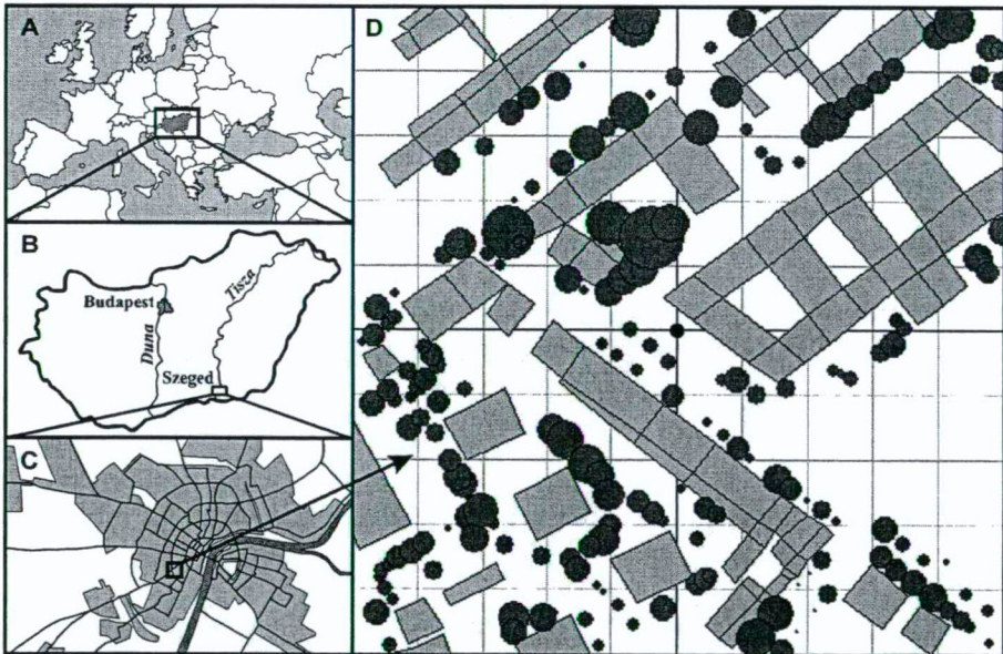
Fig. 1 Geographical location of Hungary in Europe (A), of Szeged in Hungary (B), the road network of the city (C) and the investigation area (D) with fixed measurement site in its centre (•) created by the RayMan model. The buildings are marked by light grey and trees by dark grey on the part of D.
