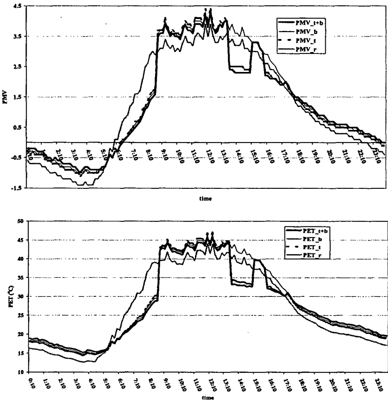
Fig. 5 Predicted Mean Vote PMV and Physiological Equivalent Temperature PET in the three urban structures and on the roof on 4 th August 2000
