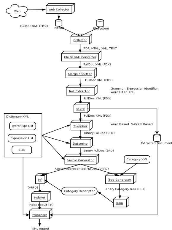
Figure 2: The document processing flow of the system
