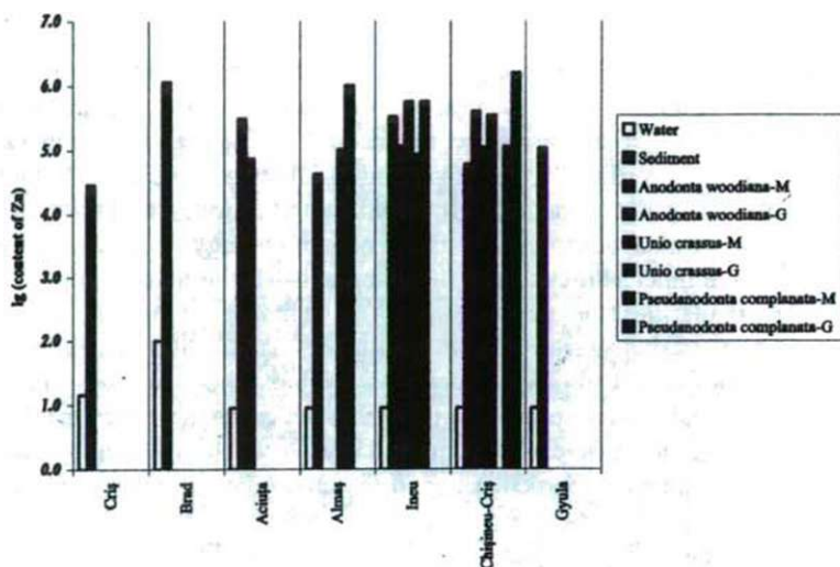
Fig. 4. Zink content in water, sediments and Unionidae mussels along the Crişul Negru, Kettős- and Hármas Kőrös Rivers Vallies
