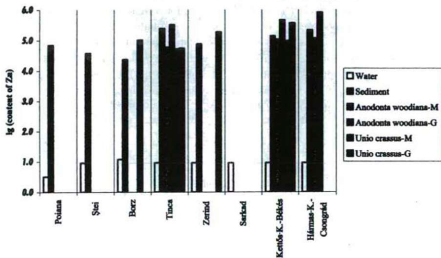
Fig. 4. Zink content in water, sediments and Unionidae mussels along the Crişul Negru, Kettős- and Hármas Kőrös Rivers Vallies
