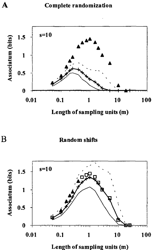
Fig. 2. Overall spatial associations (associatum) of the ten most frequent species in a xeric perennial sand grassland in Csévharaszt, detected by different neutral models: ▲ (filled triangle) significant departure of an observed value from the neutral model ( p < 0.01 ), □ (empty square) non-significant observed values, + (plus) average of the random references based on 5000 Monte-Carlo randomizations, ----- maximum of the random references, — minimum of the random references.
