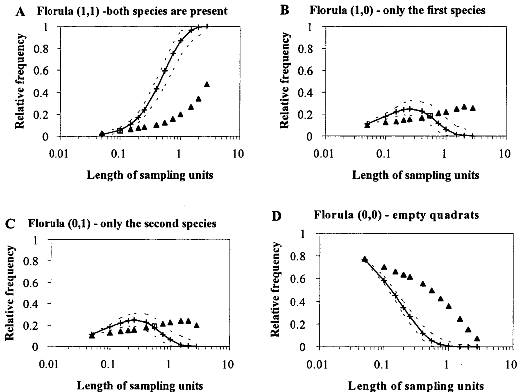
Fig. 6. The effect of within-species spatial dependence (autocorrelation) on the spatial patterns of species combinations. An example with Pattern 3, where both species are aggregated due to their limited dispersal, however, there are no interaction between them. \blacktriangle (filled triangle) significant departure of an observed value from the neutral model ( p < 0.05 ), \square (empty square) non-significant observed values, + average of the neutral model (5000 complete randomizations), ----- maximum and minimum of the random references.
