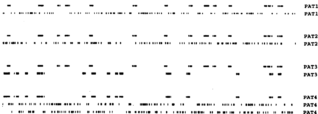
Fig. 1. Simulated spatial patterns of species along the transects (presences are marked by black dots). PAT1: species 1 is a dominant with limited dispersal, species 2 is subordinated, i.e. competitively inferior, with unlimited dispersal. PAT2: species 1 with limited dispersal, species 2 with unlimited dispersal, no competitive interaction between them. PAT3: both species with limited dispersal, no competitive interaction between them. PAT4: species 1 dominant with limited dispersal, species 2 and 3 are subordinated, i.e. competitively inferior, with unlimited dispersal. (In this paper, the association was analysed only between species 2 and 3.)
