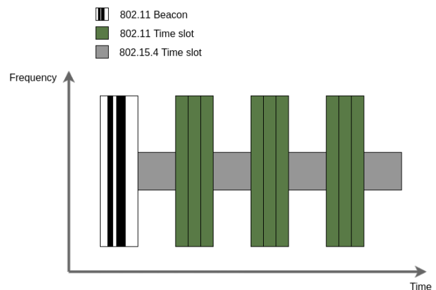
Fig. 1. Cross-technology synchronization and TMDA schedule. Each IEEE802.15.4 slot is followed by three IEEE802.11 slots
