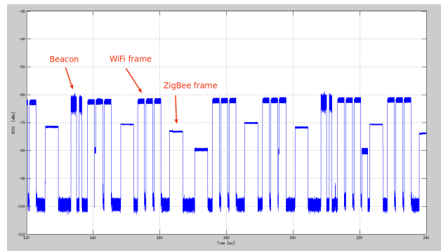
Fig. 2. Cross-technology synchronization and TDMA schedule
