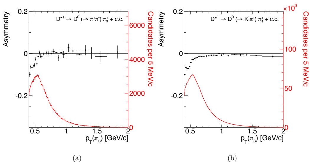
Figure 3.1: Observed asymmetry between the number of reconstructed D^{*+} and D^{*-} mesons as a function of the soft pion's transverse momentum for a pure sample of D^{*+} \rightarrow D^0(\rightarrow \pi^+\pi^-)\pi_s^+ (a) and D^{*+} \rightarrow D^0(\rightarrow K^-\pi^+)\pi_s^+ (b) decays. The soft pion transverse momentum spectrum is also shown superimposed.
