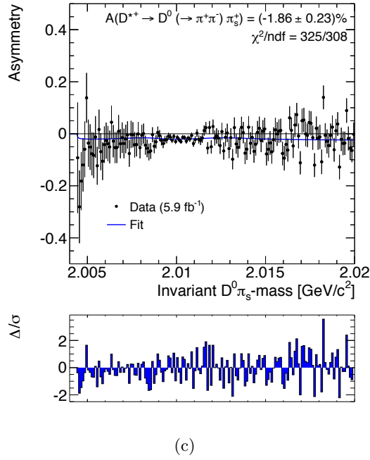
Figure 5.3: Results of the combined fit of the tagged D^0 \rightarrow \pi^+\pi^- sample. Distribution of D^0\pi_s mass for charm (a), and anticharm (b) decays, and asymmetry as a function of the mass (c). Fit results are overlaid.
