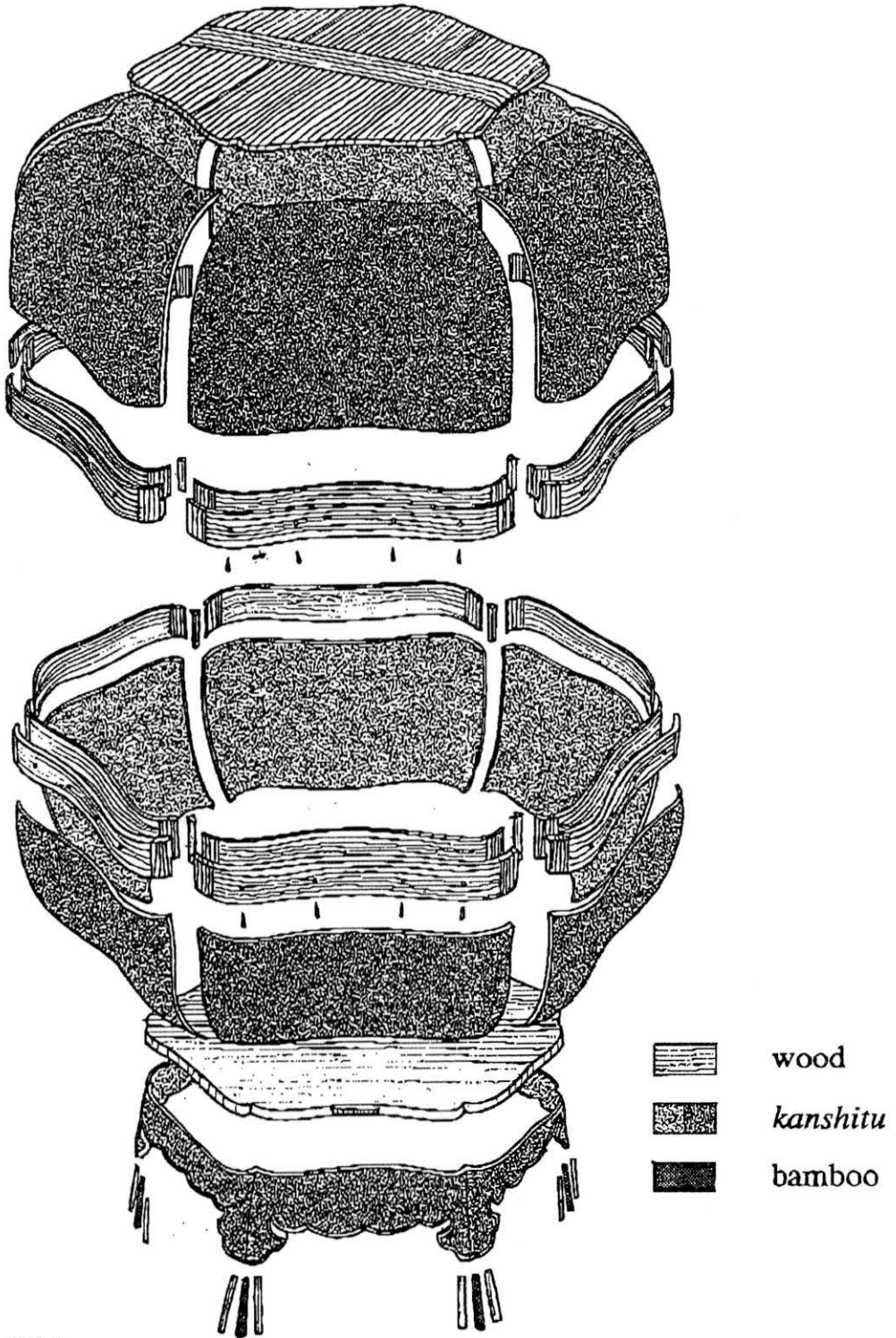
图69 素地構造図 Drawing of the structure of the substrate
