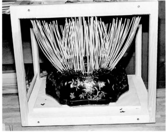
図85 螺鈿の圧着 蓋甲板 Applying pressure to the raden of the lid top
