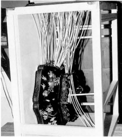
図86 螺鈿の圧着 身側板、高台 Applying pressure to the raden on the sides of the body and kodai
