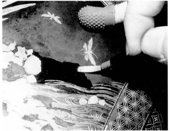
図87 漆固め 蓋甲板 Urushi consolidation of the lid top
