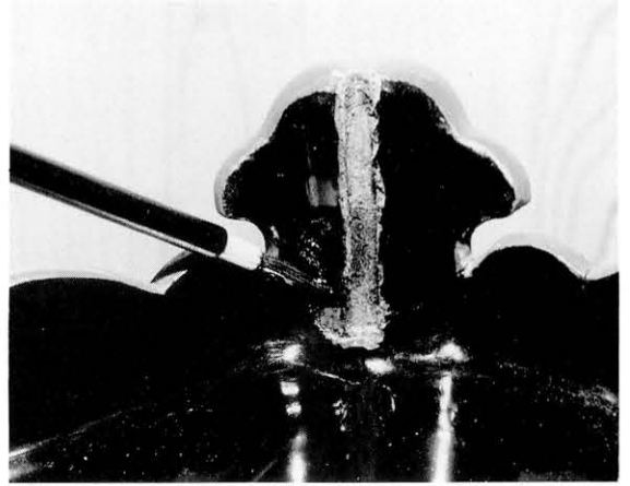
図79 麦漆の含浸 刳足亀裂部分 Impregnating mugi urushi to the cracks of kuriashi
