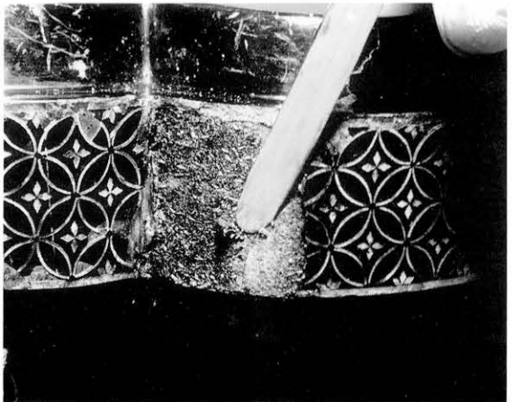
図95 下地欠損部の刻字付け Applying kokuso to the missing parts of the foundation
