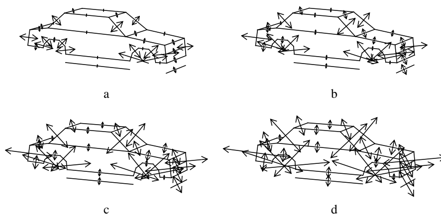
Figure 3 Search regions (perpendicular in the image to the projected model lines) determined by \pm 3 sd of the estimated filter covariance for forward predictions of (a,b,c,d) 0, 5, 10 and 15 fields (@ 50 Hz).
