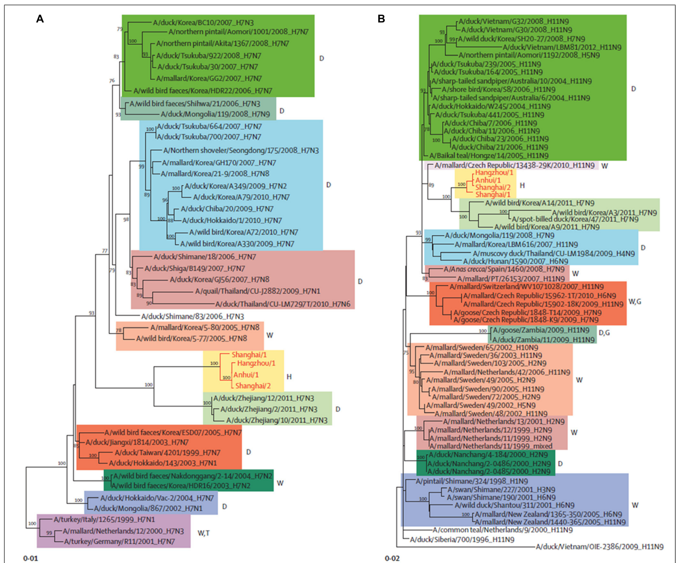
FIGURE 2 | Phylogenetic trees of H7 (A) and H9 (B). The H7N9 viruses are shown by red lines and text. D, duck; W, wild bird; H, human being; T, turkey; G, goose. Adapted from Liu et al. (2013a).
